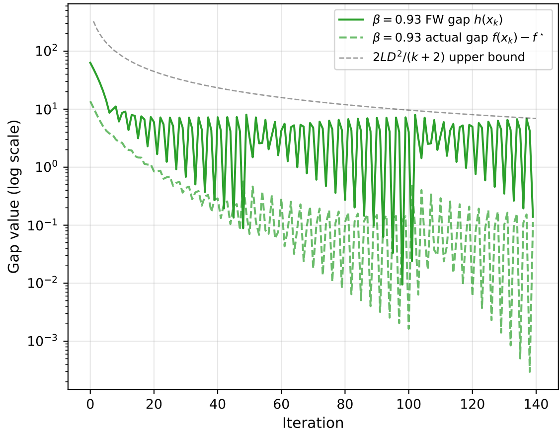
FW gap as certificate: boundary case
