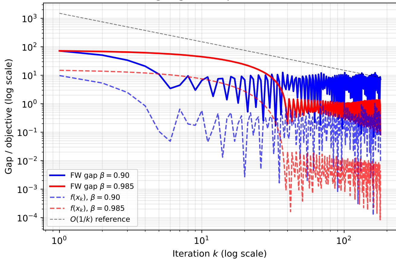
Log-Log: FW Gap vs Iteration
