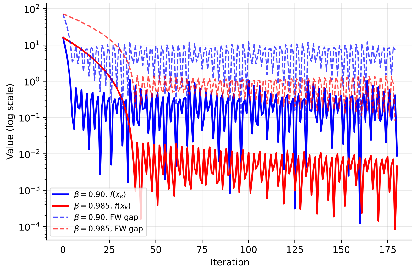
Q6: f(x_k) and Frank--Wolfe Gap \nabla f^T(x - z)
