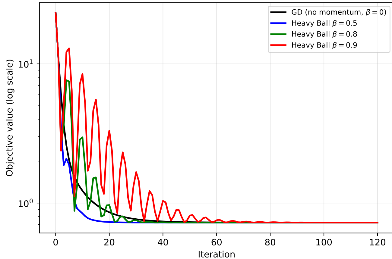
Effect of Momentum \beta on Heavy Ball (Bench. B)
