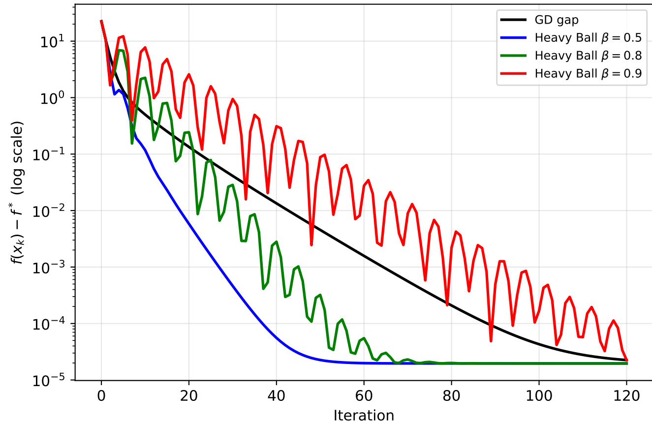
Function-Value Gap: GD vs Heavy Ball (Bench. B)
