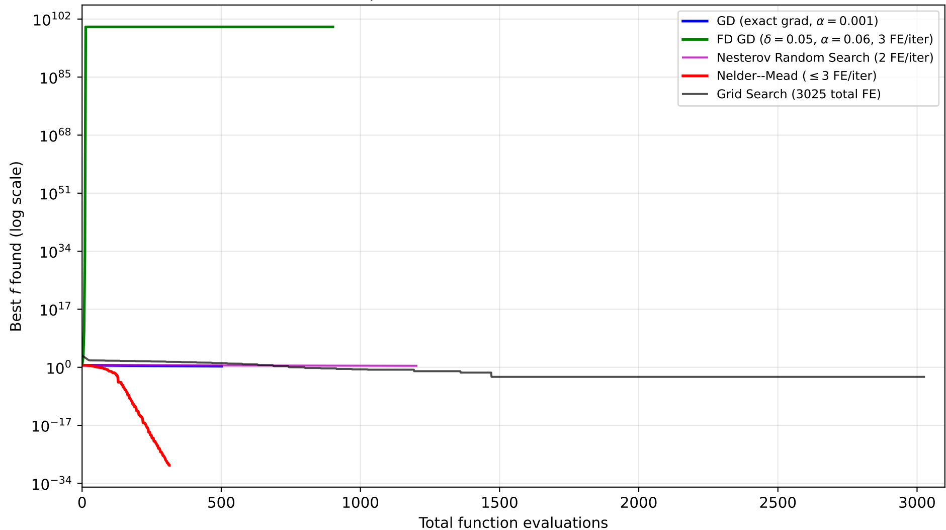
Q4: Method Comparison on Rosenbrock — Per Function Evaluation
