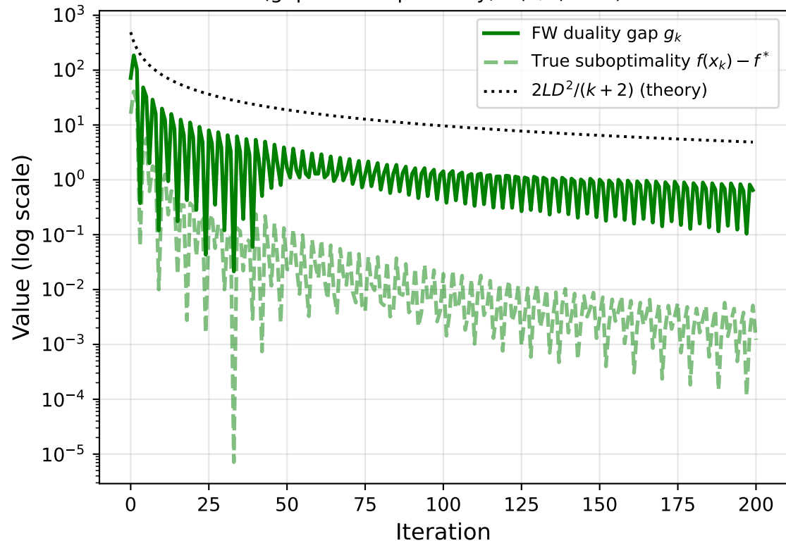
FW Duality Gap vs True Suboptimality (gap \geq suboptimality, O(1/k) rate)
