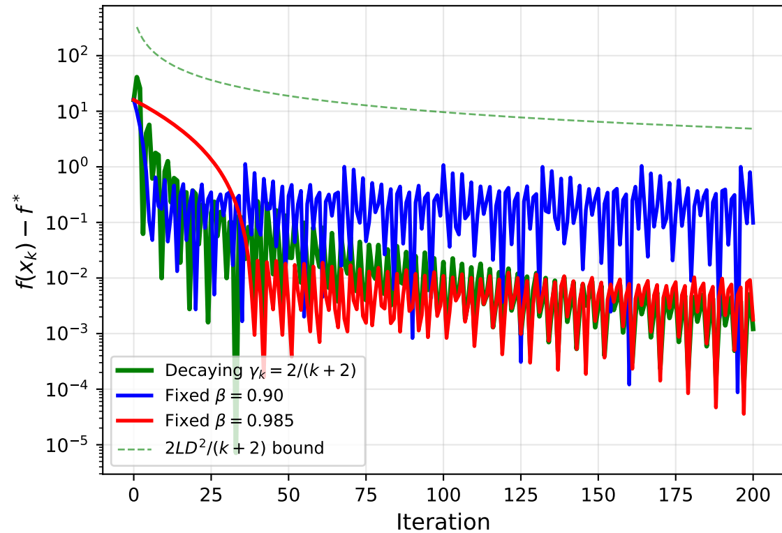
Frank--Wolfe: Decaying vs Fixed Step (interior optimum, Case II)
