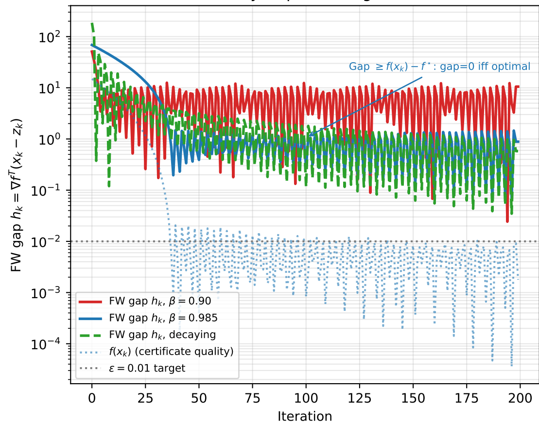
Frank-Wolfe Duality Gap (Convergence Certificate)
