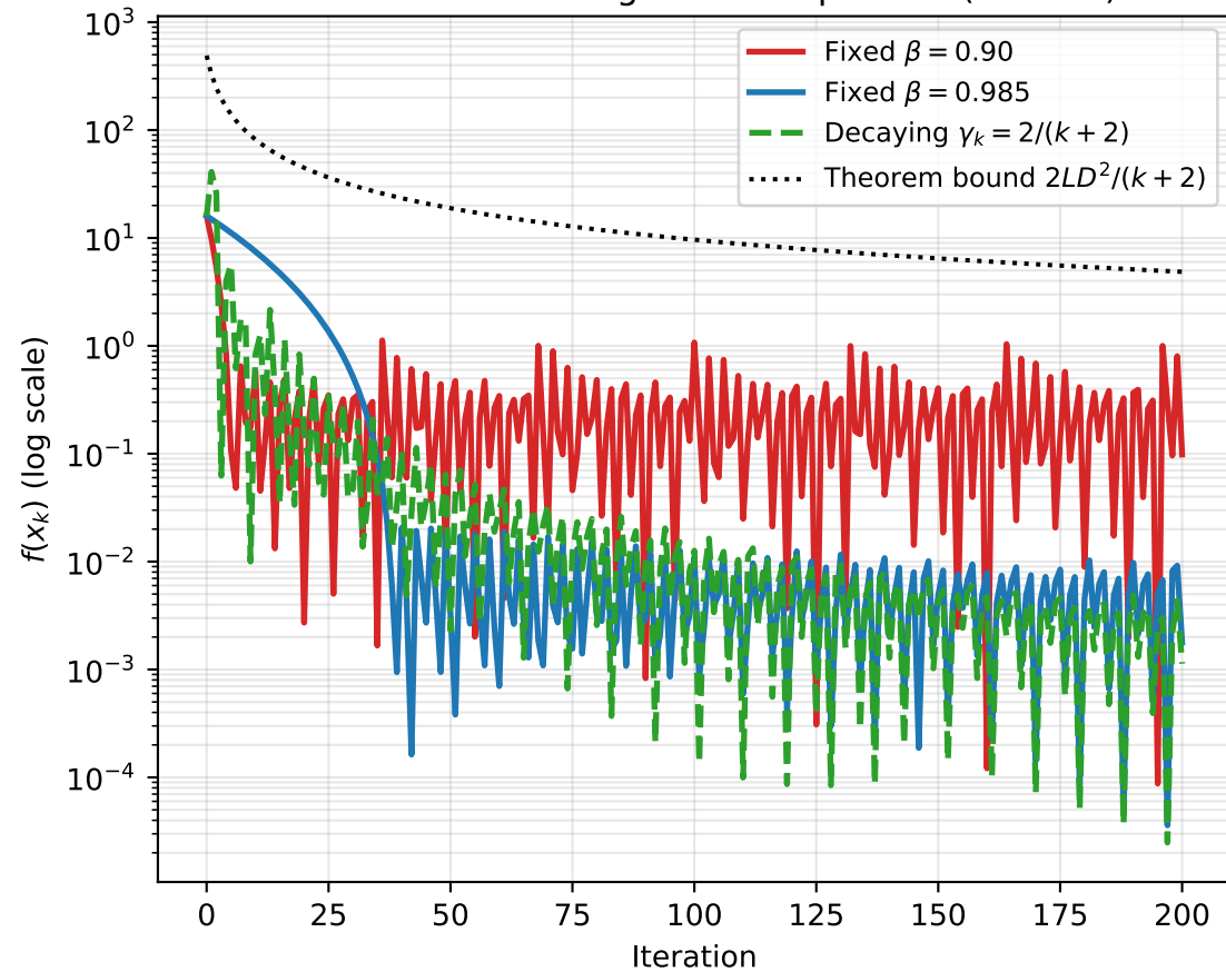
Frank-Wolfe Convergence Comparison (Interior)
