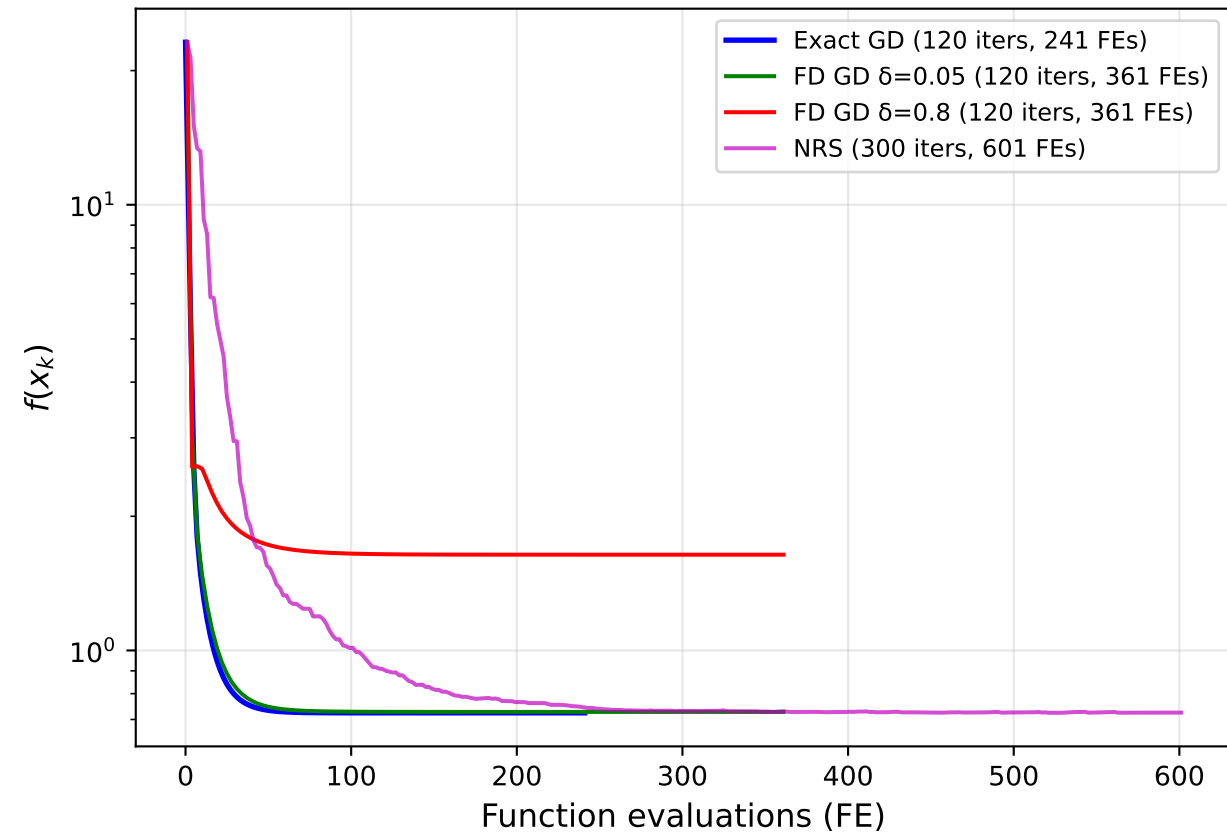
Oracle Complexity: Convergence vs FE (accounts for per-iteration cost)
