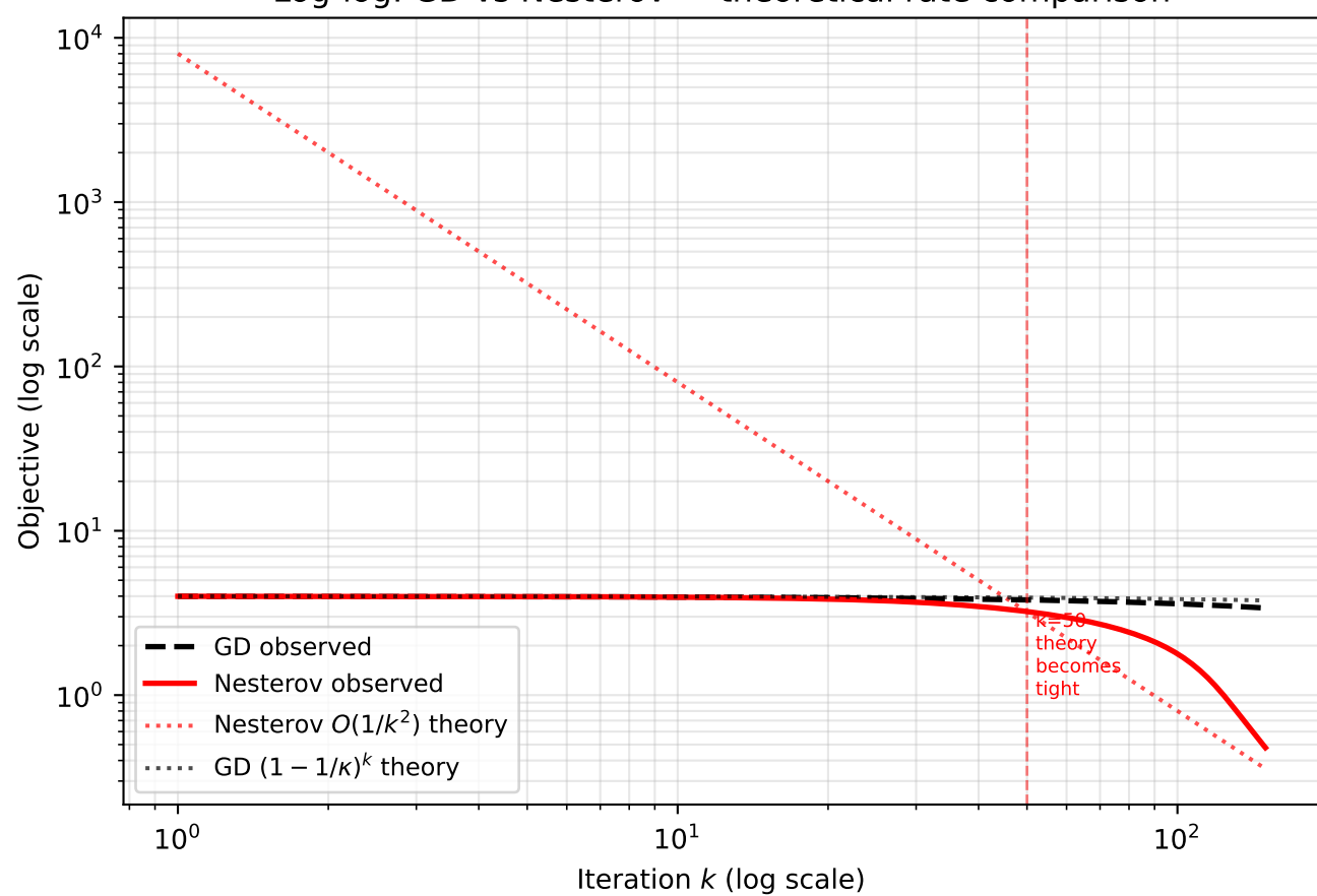
Log-log: GD vs Nesterov — theoretical rate comparison
