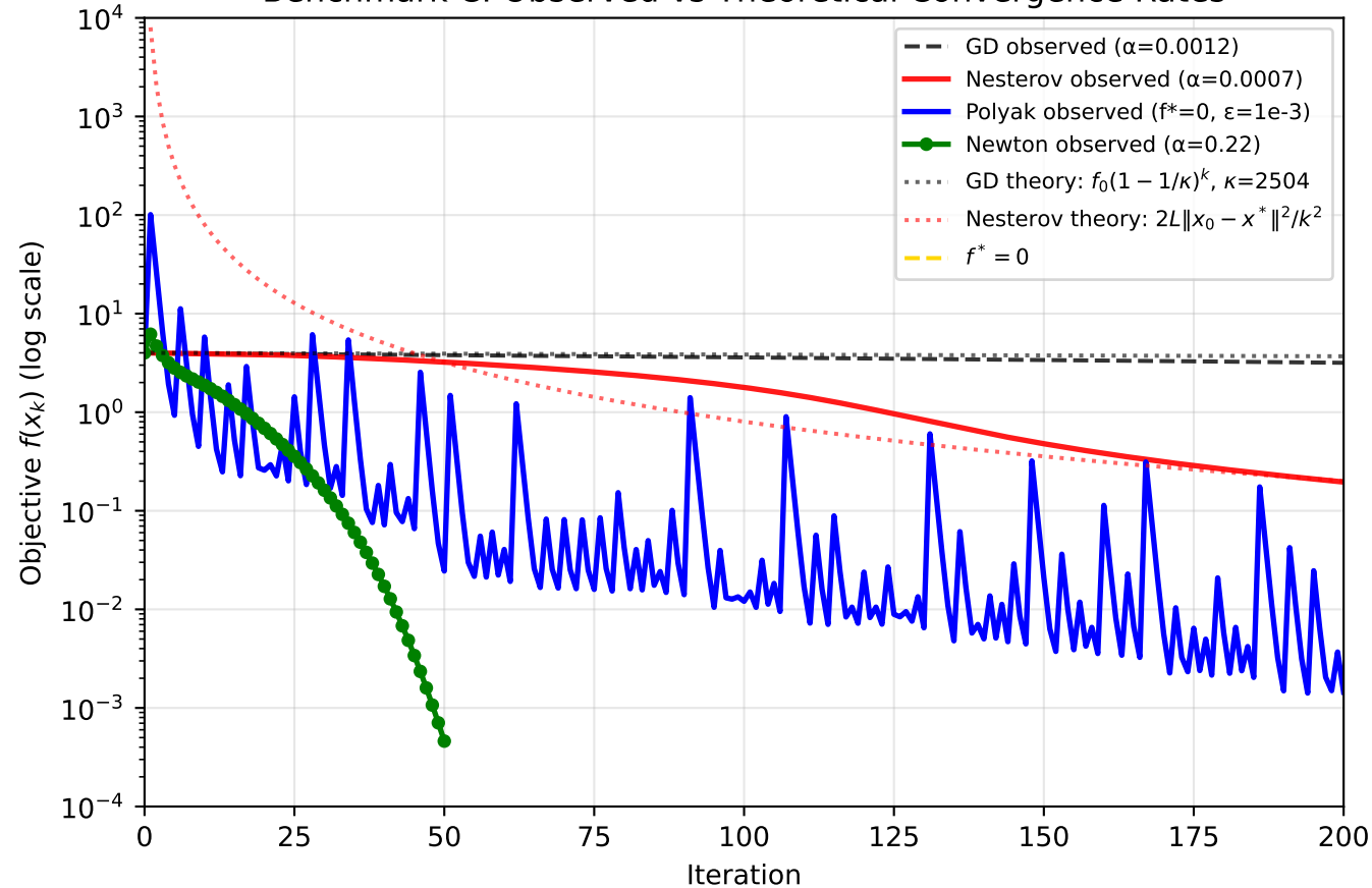
Benchmark C: Observed vs Theoretical Convergence Rates
