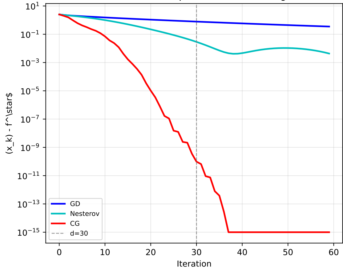
First 60 iterations (super-linear CG convergence)
