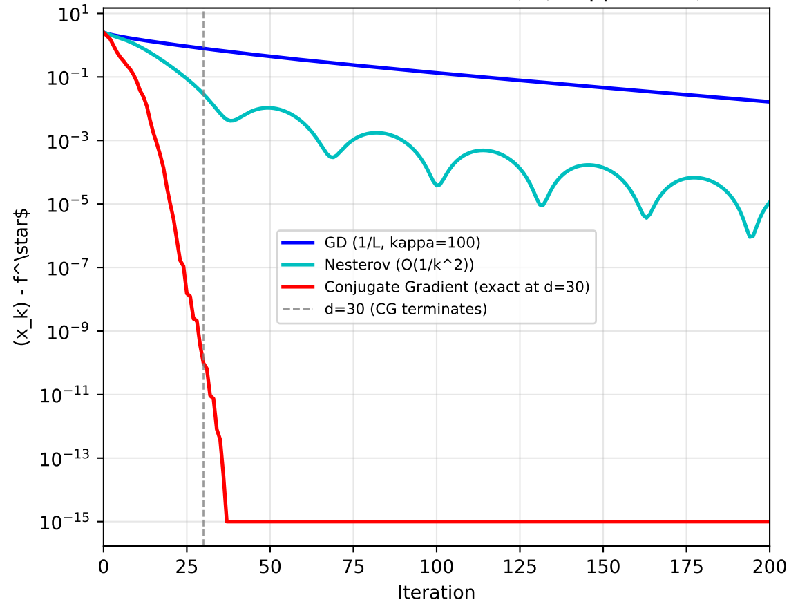
CG vs First-Order Methods ( =30 , \kappa=100 )
