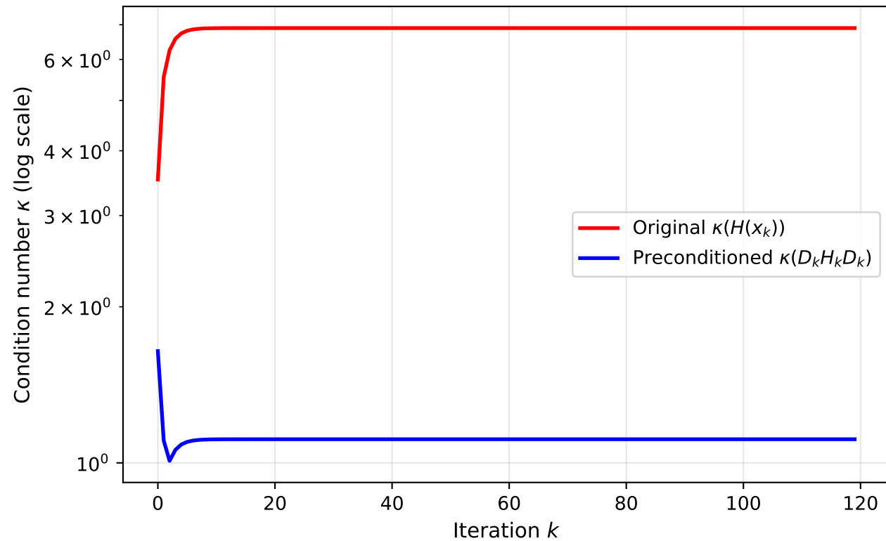
Adagrad's Implicit Preconditioning Effect (Benchmark B, Hessian condition number)
