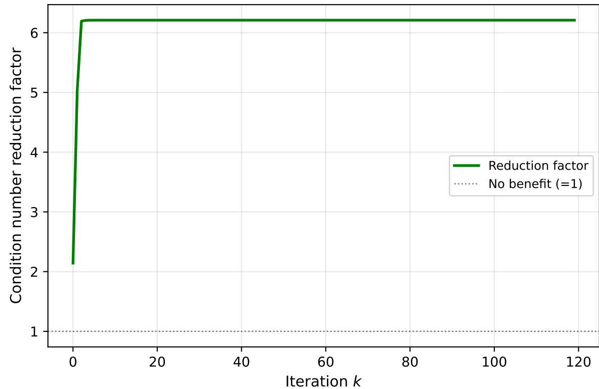
Preconditioning Factor \kappa(H)/\kappa(D_k H D_k) (higher = more benefit from preconditioning)
