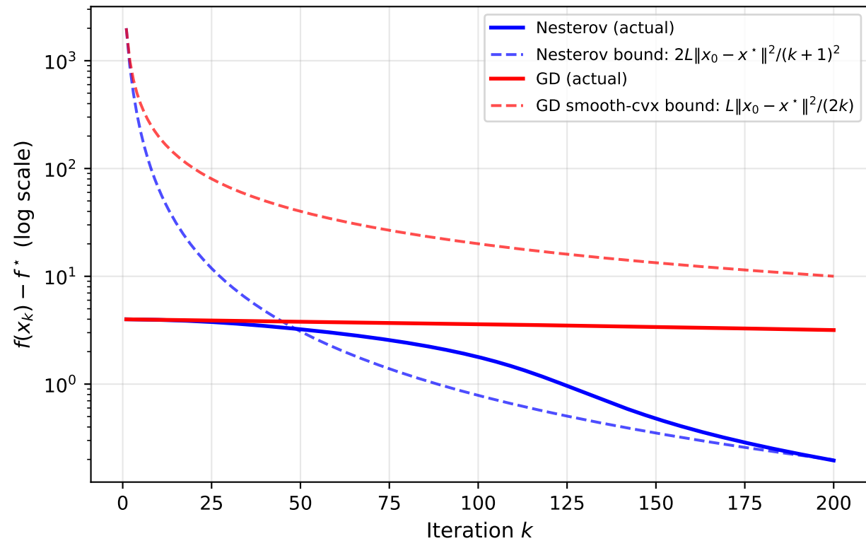
Nesterov vs GD: Actual vs Theoretical Bounds (Benchmark C, L = 1001.6 , \|x_0 - x^*\|^2 = 4 )
