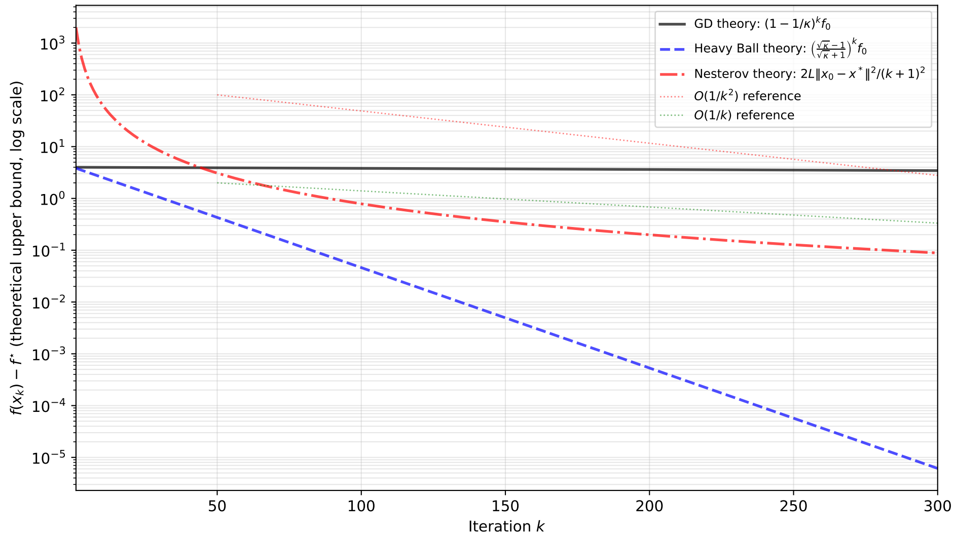
Theoretical Convergence Rate Comparison on Rosenbrock ( \kappa \approx 2009 )
