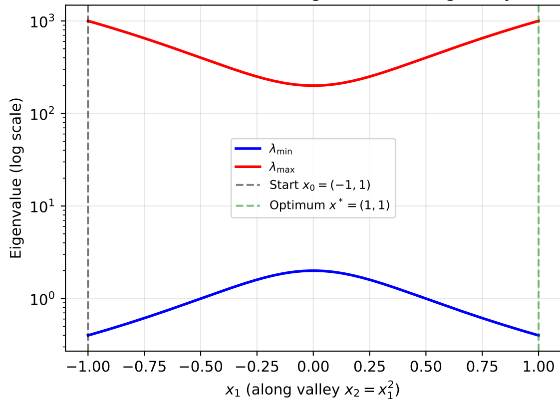
Rosenbrock Hessian Eigenvalues Along Valley
