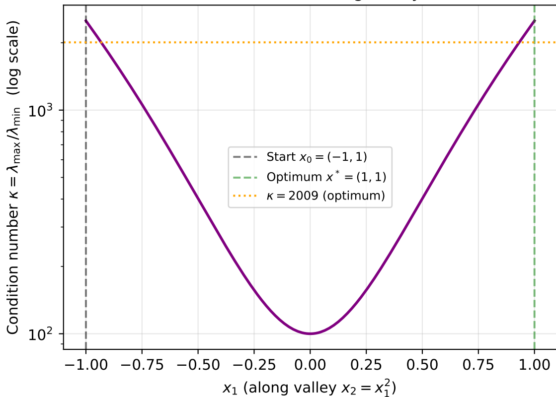
Condition Number Along Valley Floor
