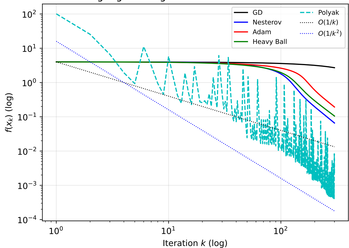
Log-log convergence rates on Benchmark C
