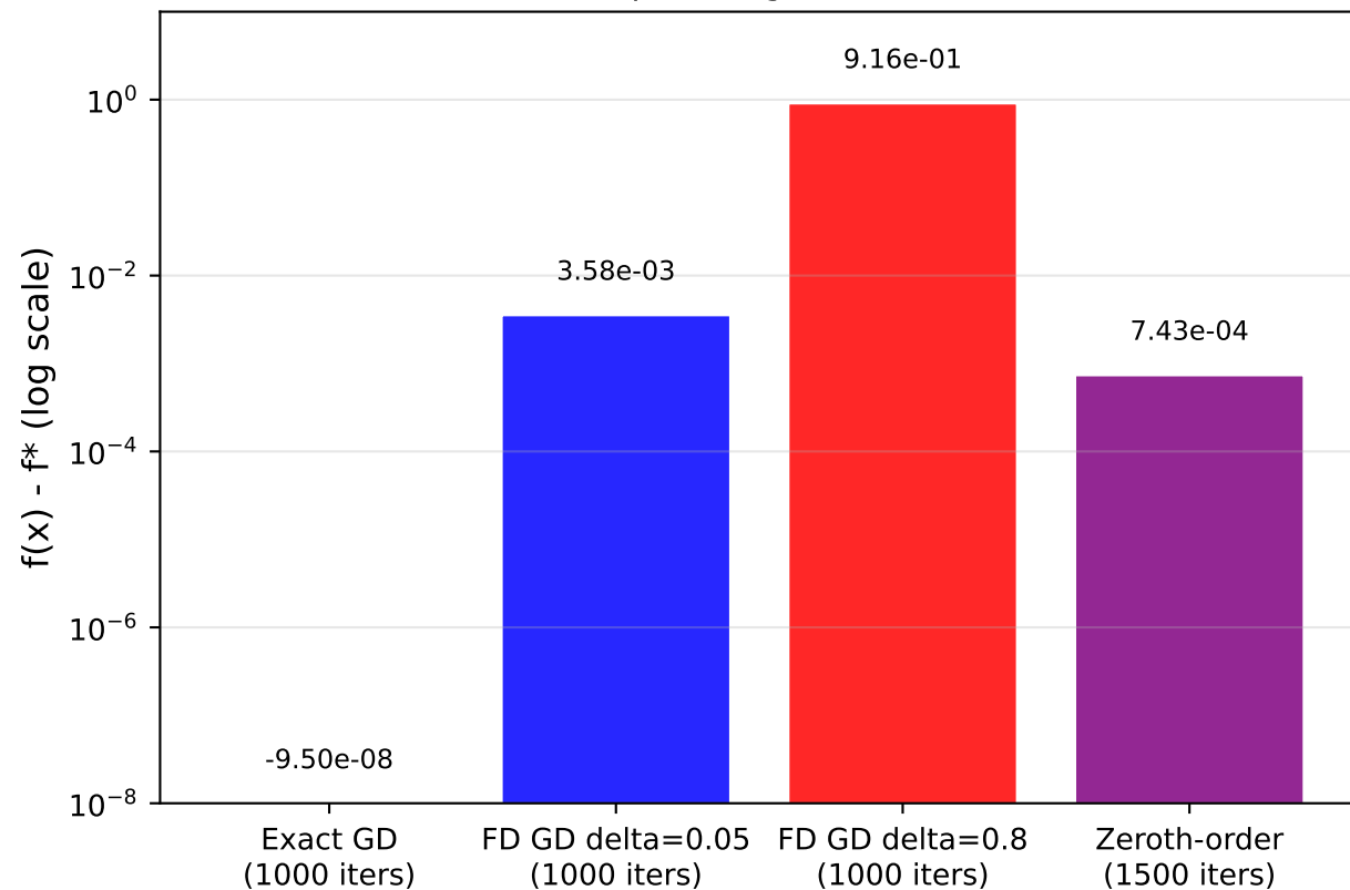
Benchmark B: Equal Budget (3000 total FE, d=2 )
