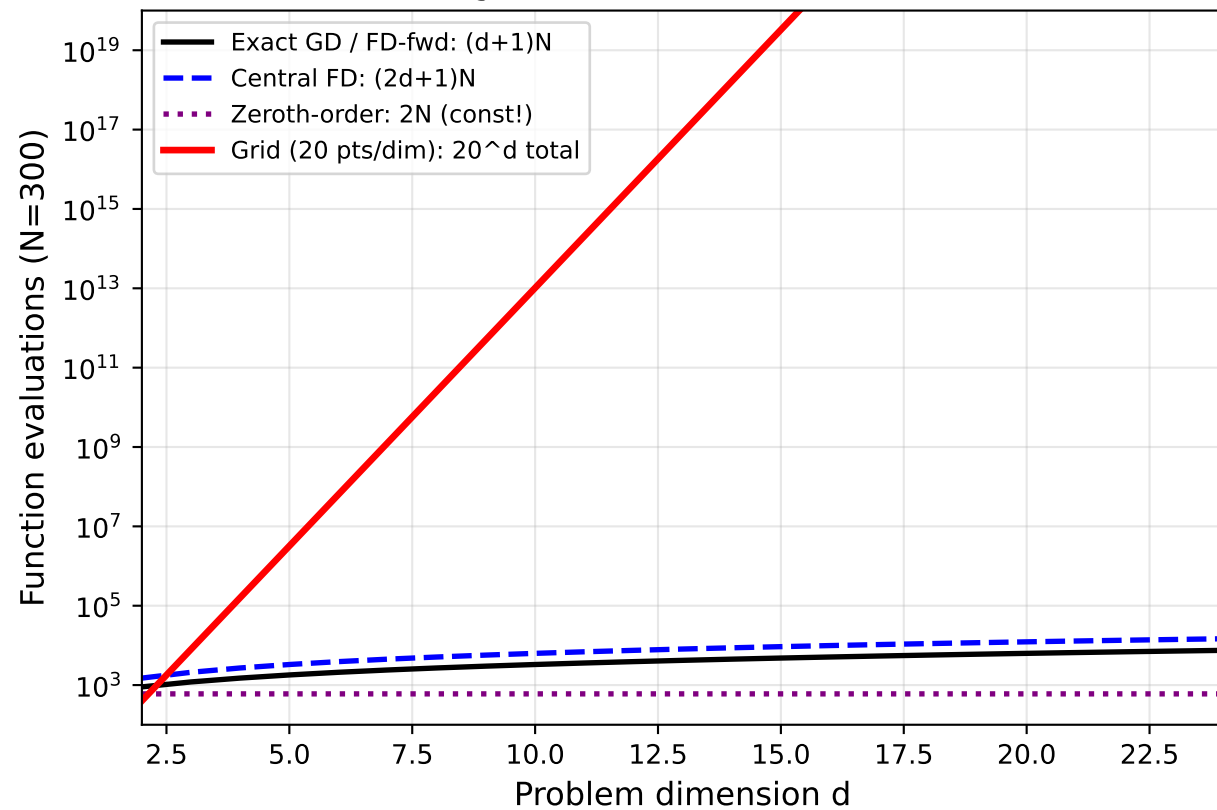
FE Scaling: First-Order vs Zeroth-Order vs Grid
