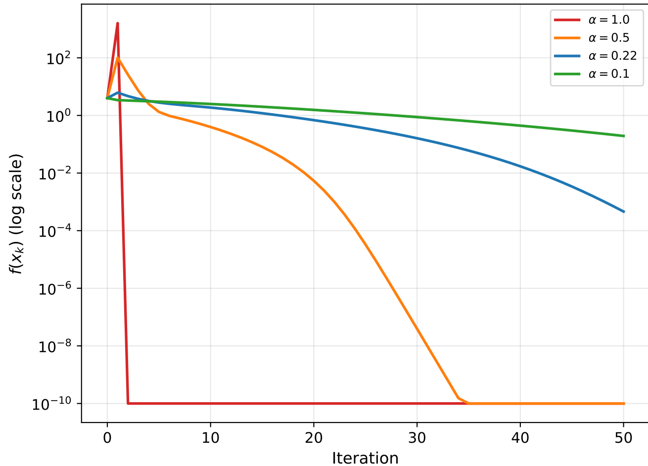
Newton Convergence for Different Damping \alpha (Rosenbrock, 50 iterations)
