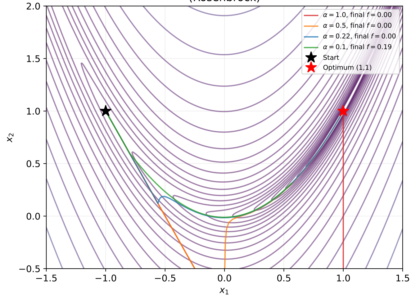
Newton Trajectories for Different Damping \alpha (Rosenbrock)
