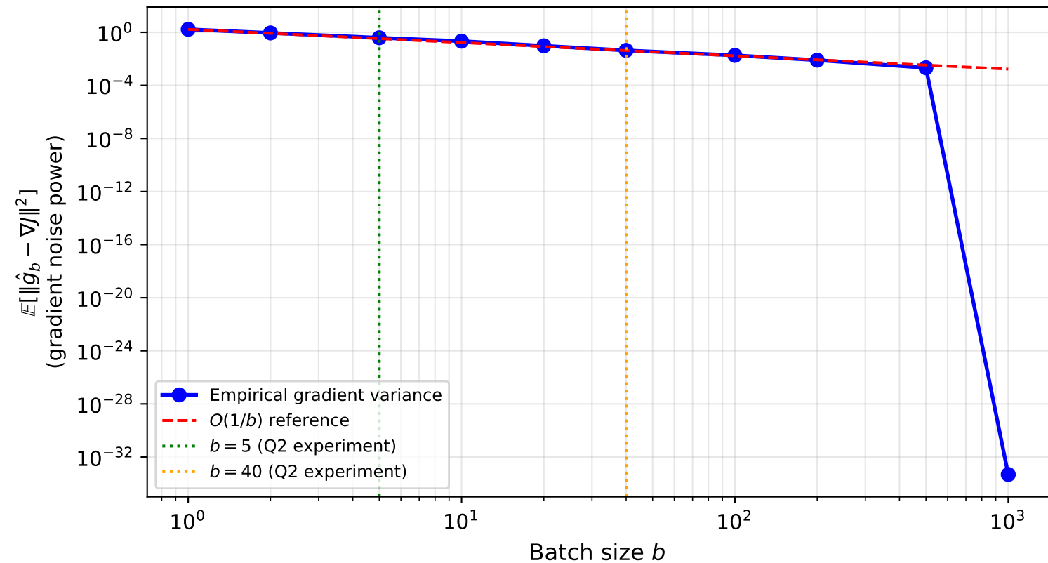
Mini-Batch SGD: Gradient Variance vs Batch Size (Benchmark A, at \hat{\theta}_{\text{OLS}} , n = 200 trials)
