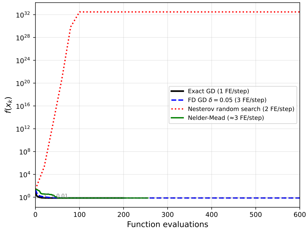
Oracle Complexity: Function Evals to Convergence (Benchmark B)
