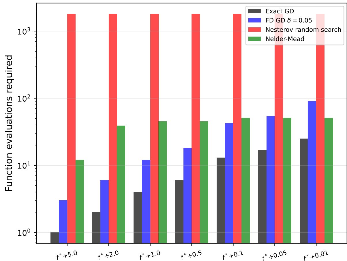
FEs to Reach f(x) \leq f^* + \tau (Benchmark B)
