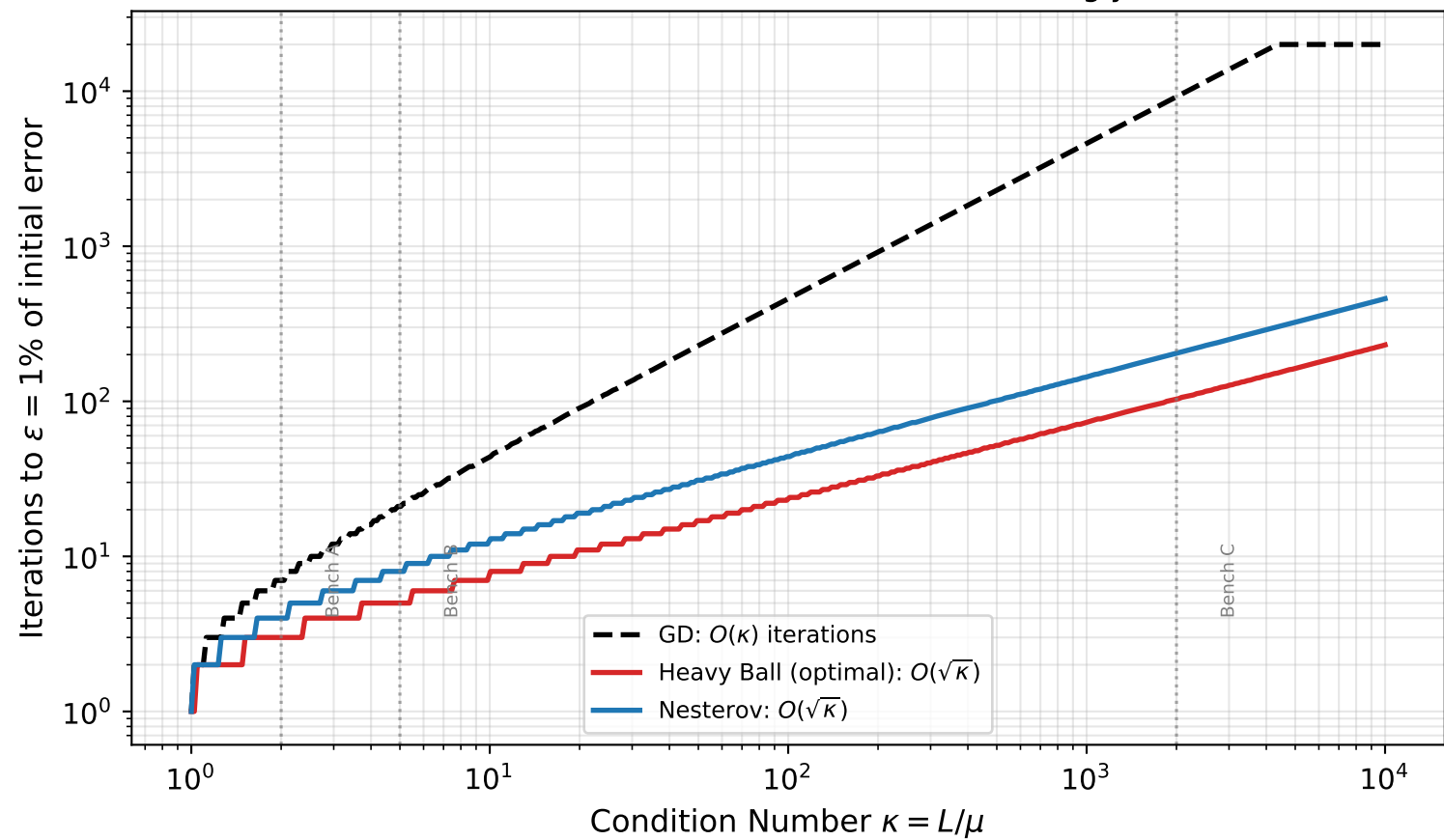
Theoretical Iterations vs Condition Number (strongly convex)
