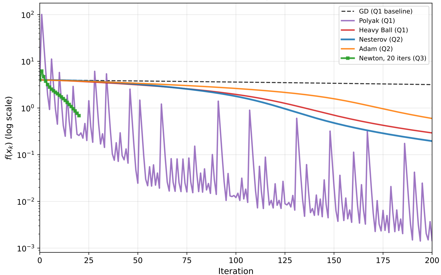
Cross-Question Rosenbrock Comparison ( \kappa \approx 2000 )
