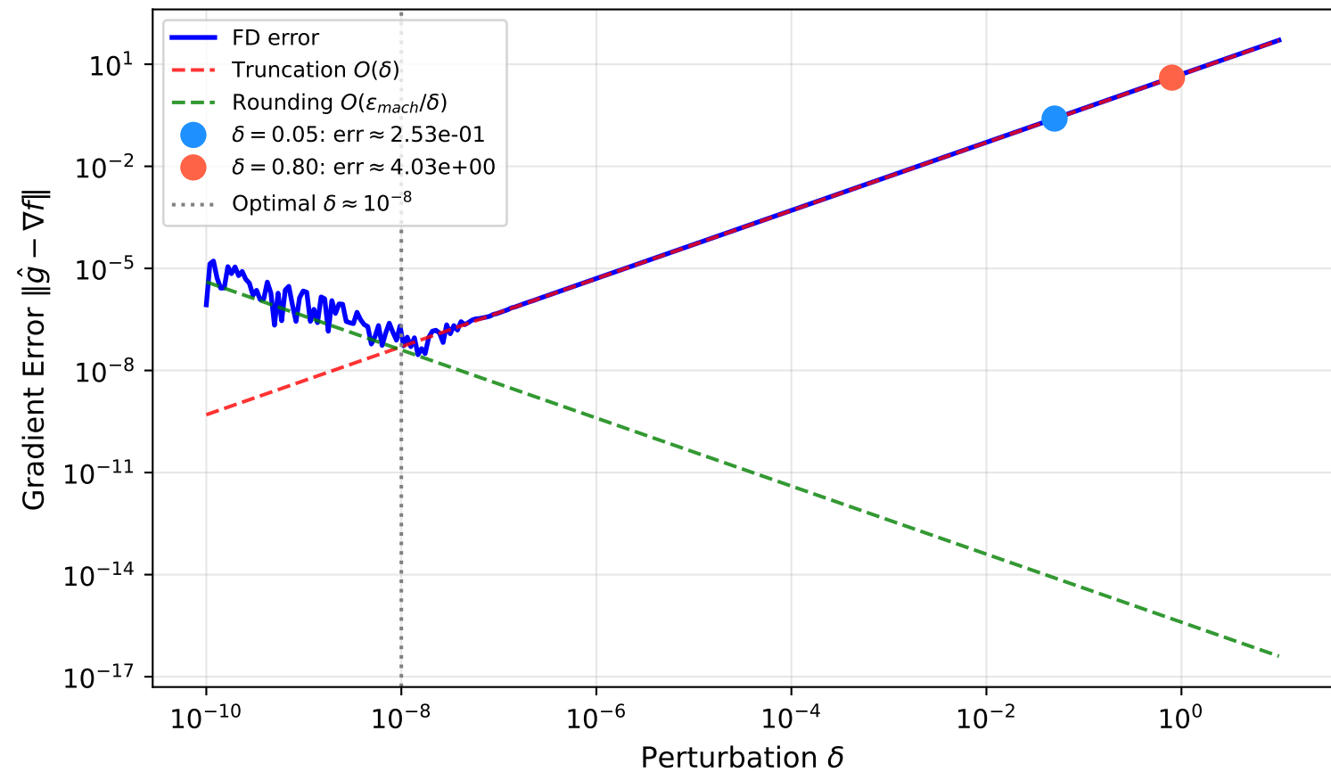
Finite Difference Error vs Perturbation Size (Benchmark B)
