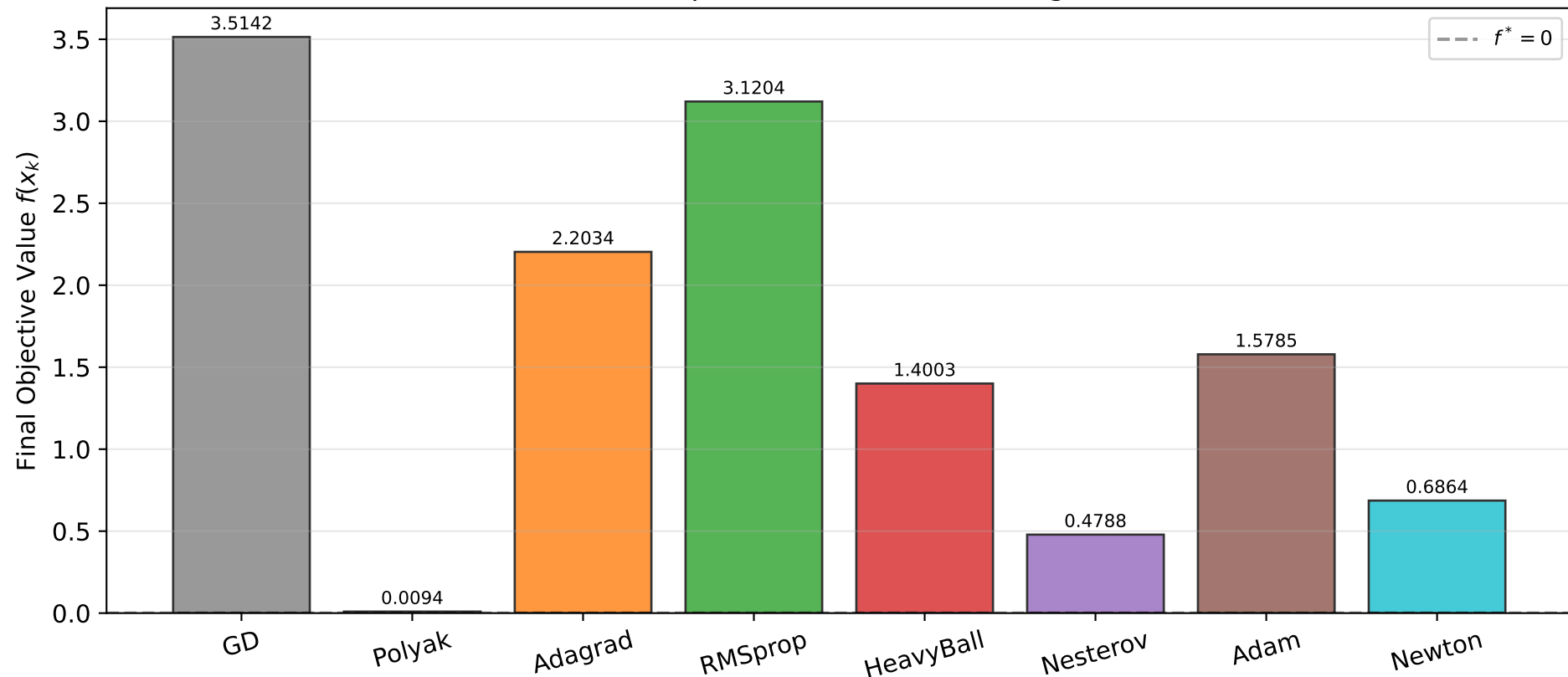
All Methods: Final Objective on Benchmark C (Rosenbrock) after equivalent evaluation budget
