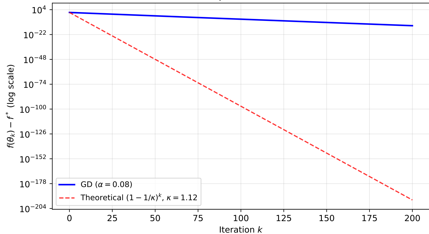
Q1: GD Linear Convergence on Benchmark A ( L = 1.033 , \mu = 0.925 , \kappa = 1.12 )
