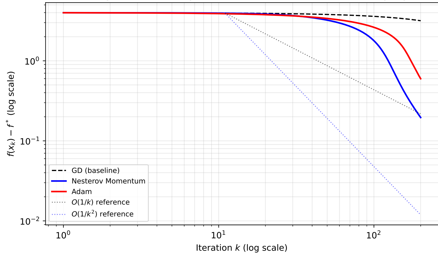
Q2: Convergence Rate Analysis — Benchmark C (Rosenbrock), log-log scale
