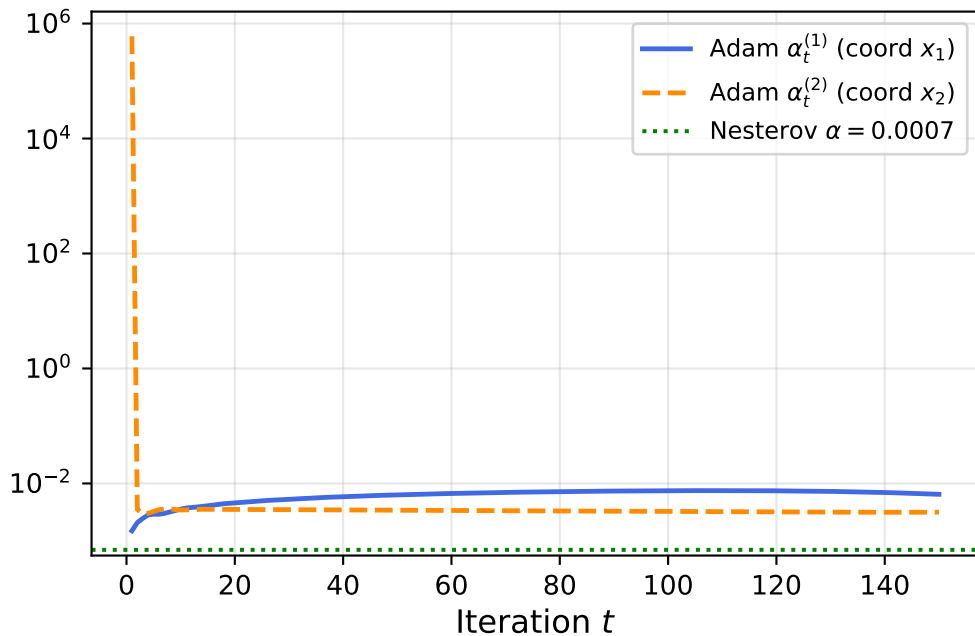
Adam per-coordinate effective step size (Rosenbrock, Benchmark C)
