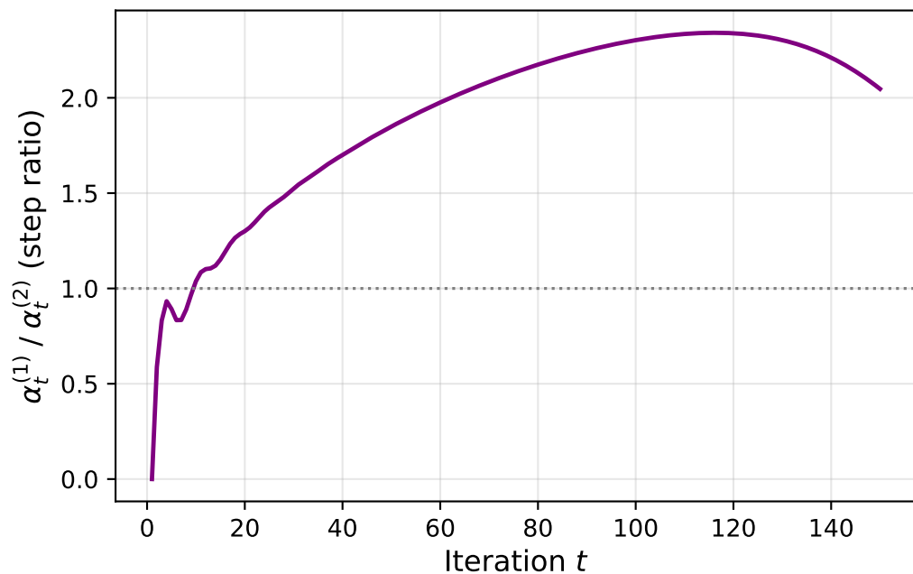
Ratio of Adam step sizes ( x_1 coord / x_2 coord)
