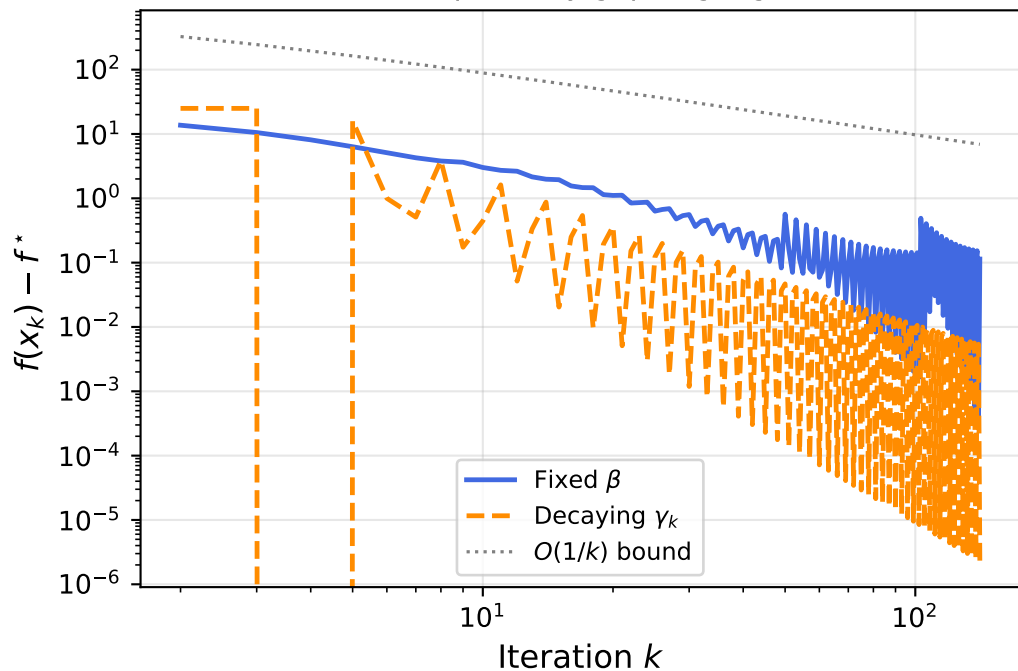
Suboptimality gap (log-log)
