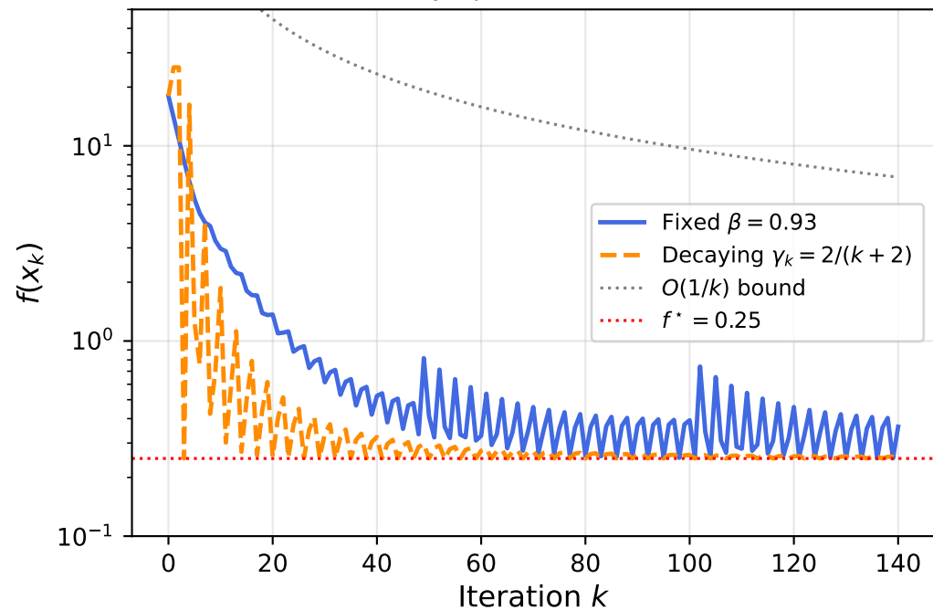
FW: fixed vs. \ decaying step (boundary optimum, Benchmark)
