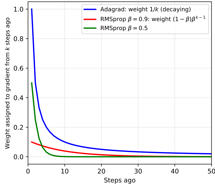
Adagrad vs. RMSprop: Gradient History Weighting
