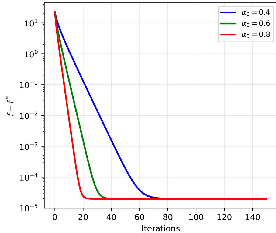
Adagrad: Effect of Base Learning Rate
