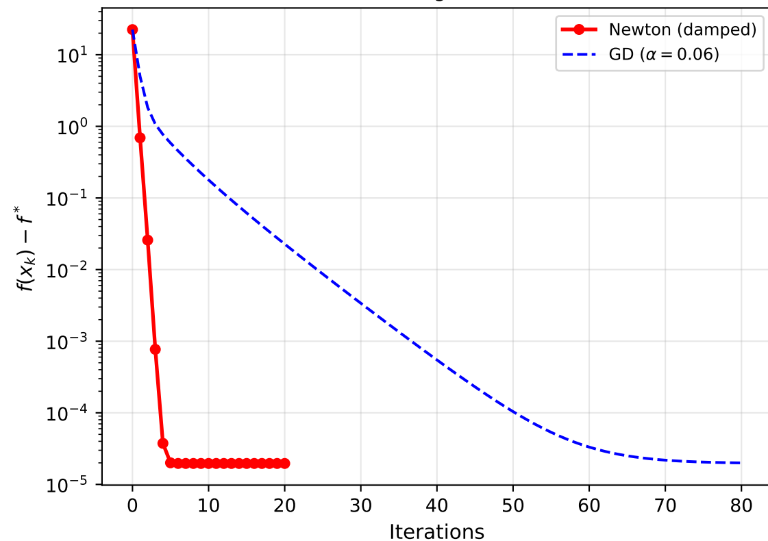
Newton vs. GD Convergence on Benchmark B
