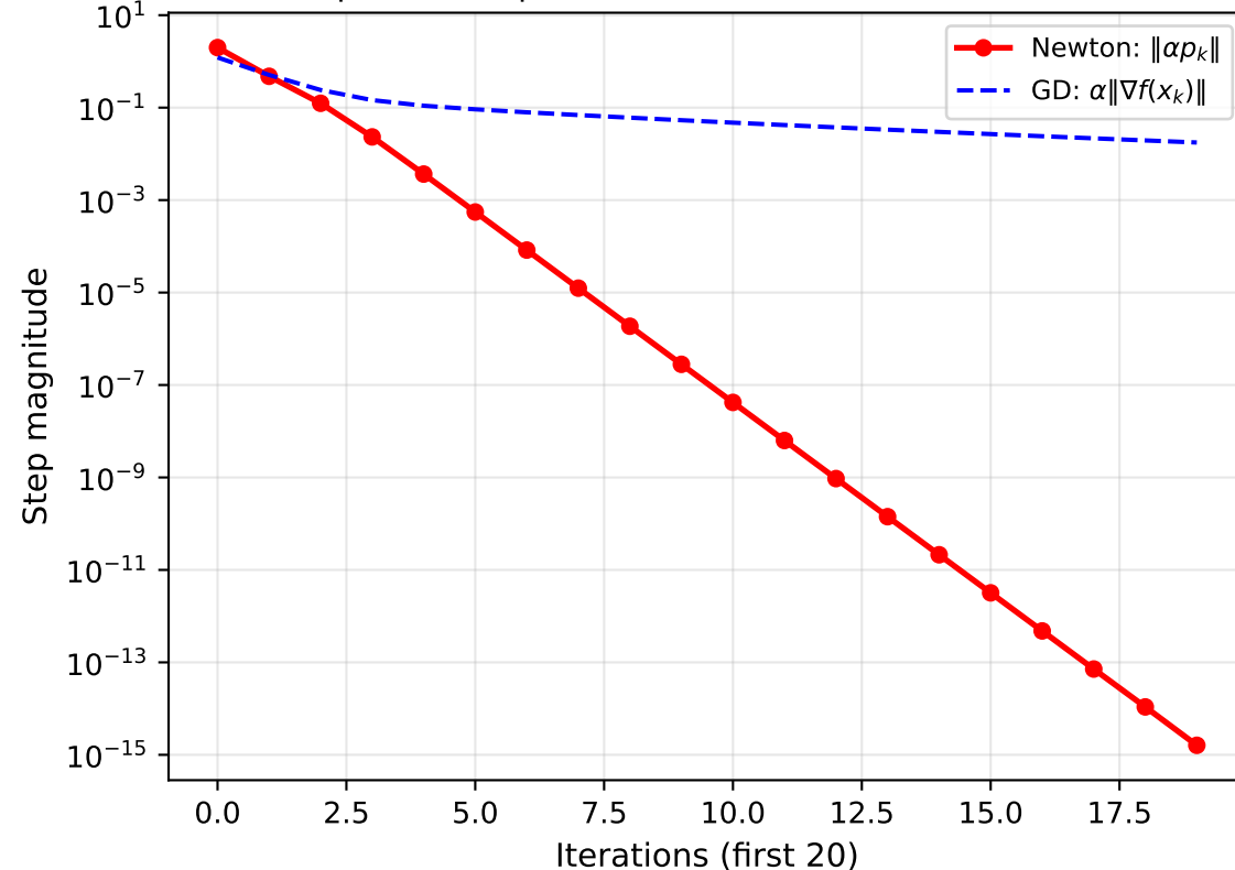
Step Size Comparison: Newton vs. GD (first 20 iters)
