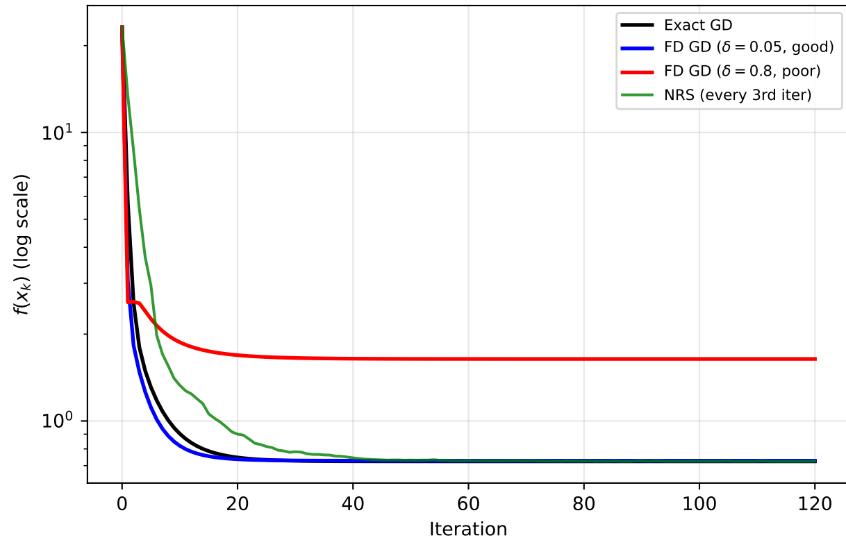
Convergence per Iteration
