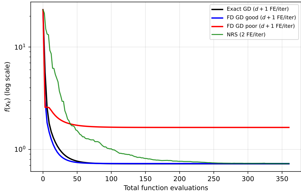
Convergence per Function Evaluation (Fair cost comparison, same budget)
