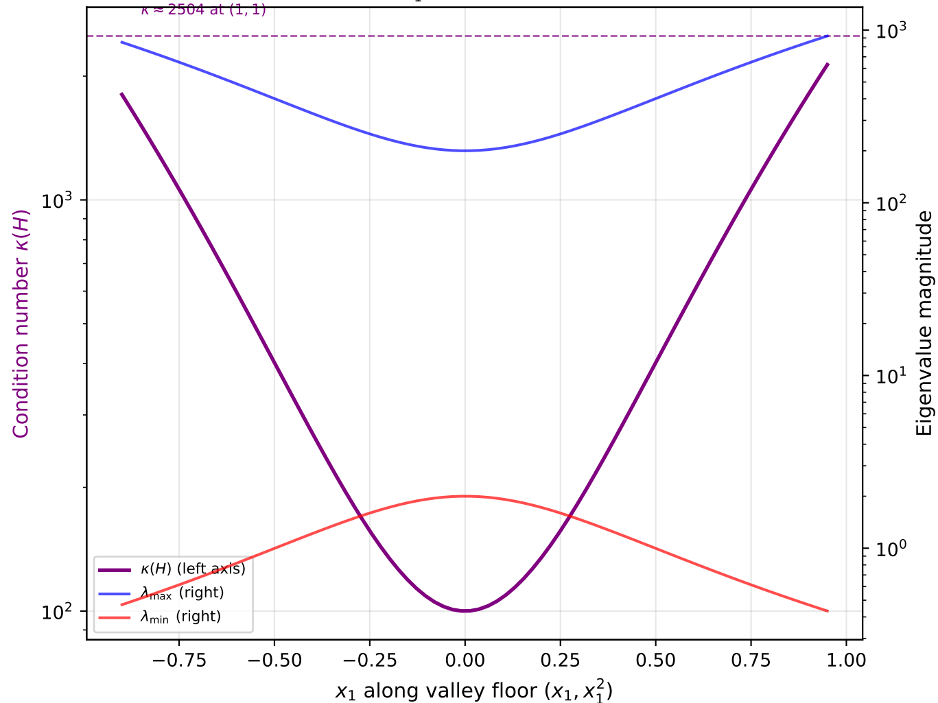
Hessian Eigenvalues Along Valley Floor
