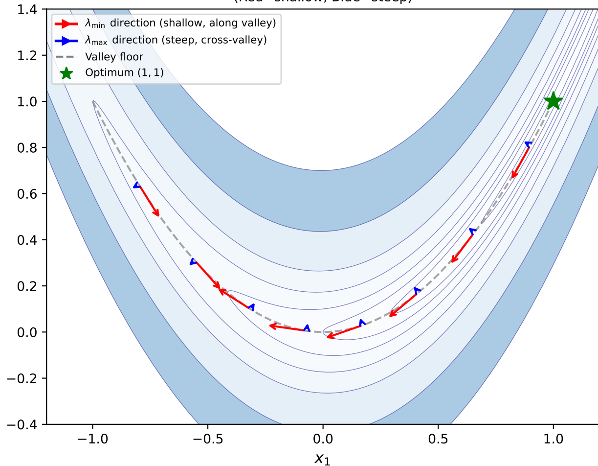
Rosenbrock: Hessian Eigenvectors Along Valley (Red=shallow, Blue=steep)
