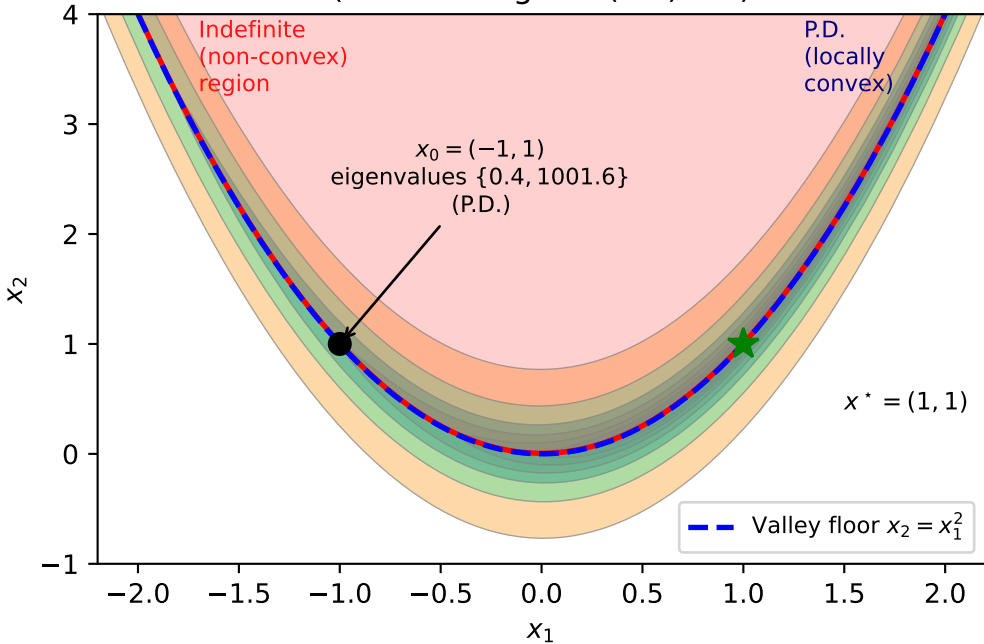
Rosenbrock non-convexity regions (red shading: \det(\nabla^2 f) < 0 )
