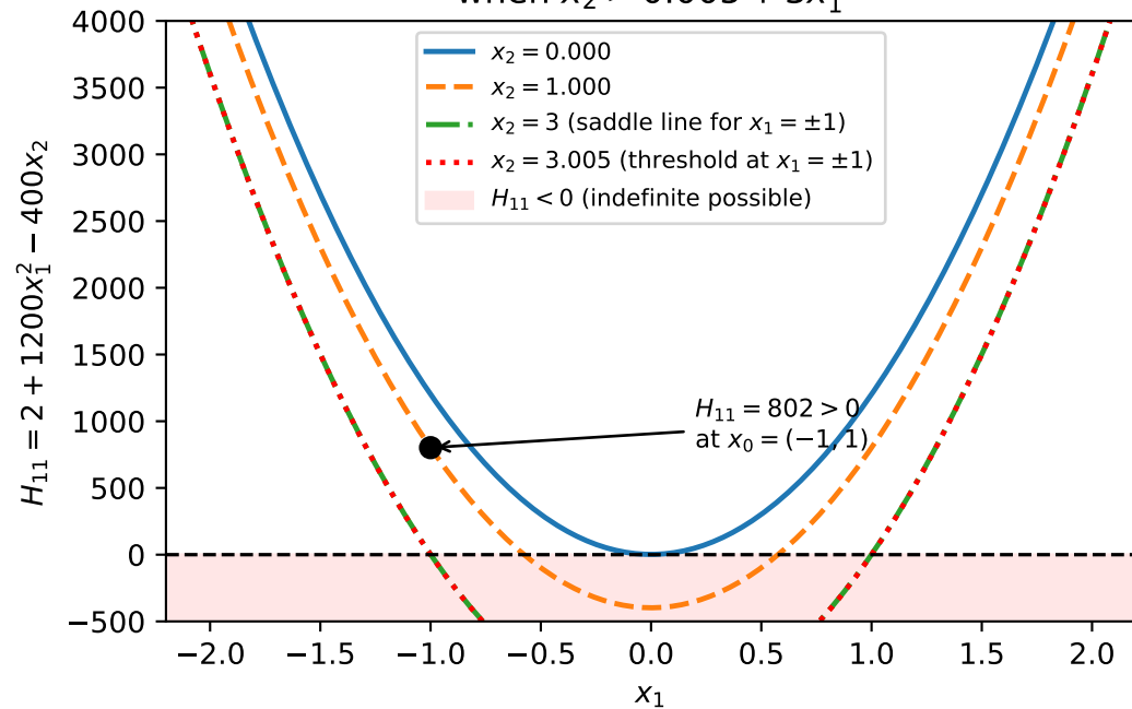
H_{11} at fixed x_2 : indefinite region when x_2 > 0.005 + 3x_1^2
