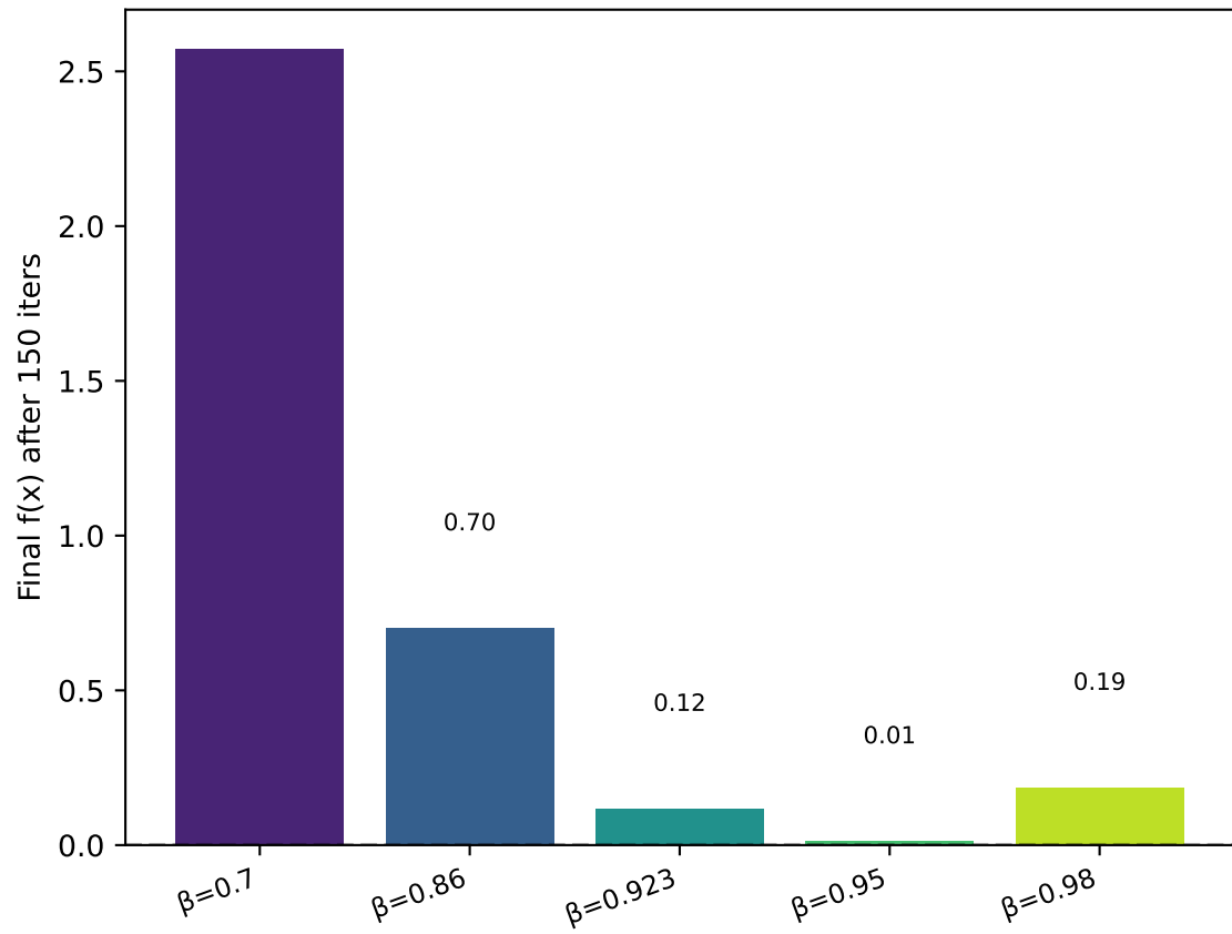
Heavy Ball: final objective vs \beta
