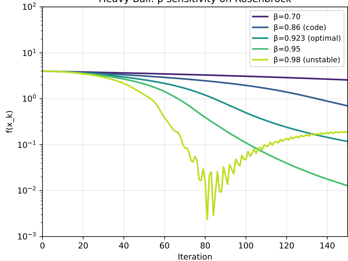
Heavy Ball: \beta sensitivity on Rosenbrock
