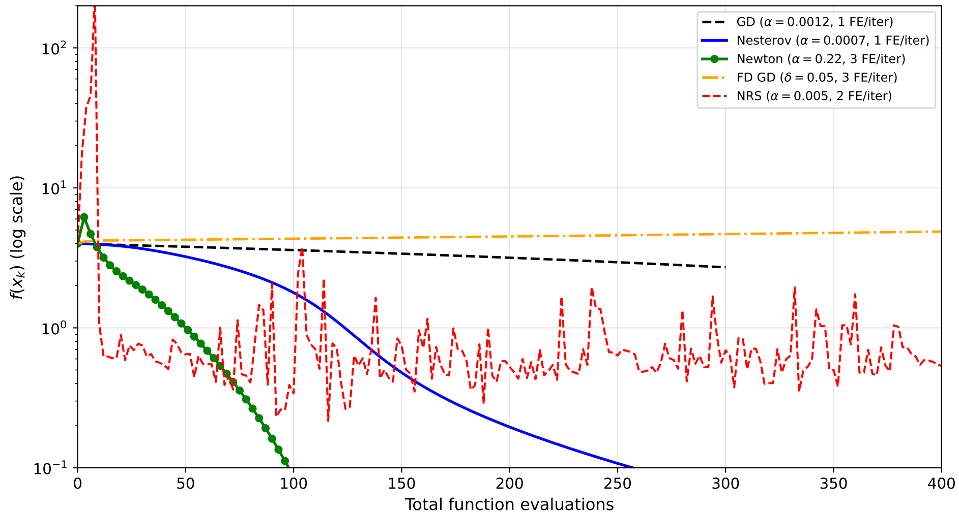
Method Comparison on Rosenbrock: Equal Function-Evaluation Budget ( d = 2 , starting from (-1, 1) , each method uses its natural FE/iter cost)
