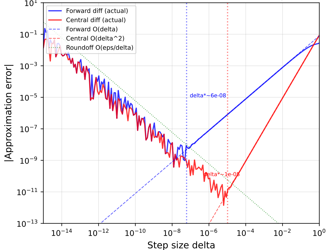
Forward vs Central Finite Difference Accuracy
