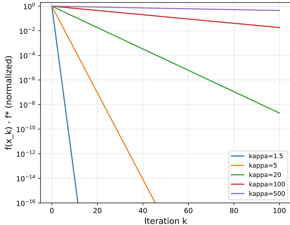
GD Convergence Rate vs Condition Number
