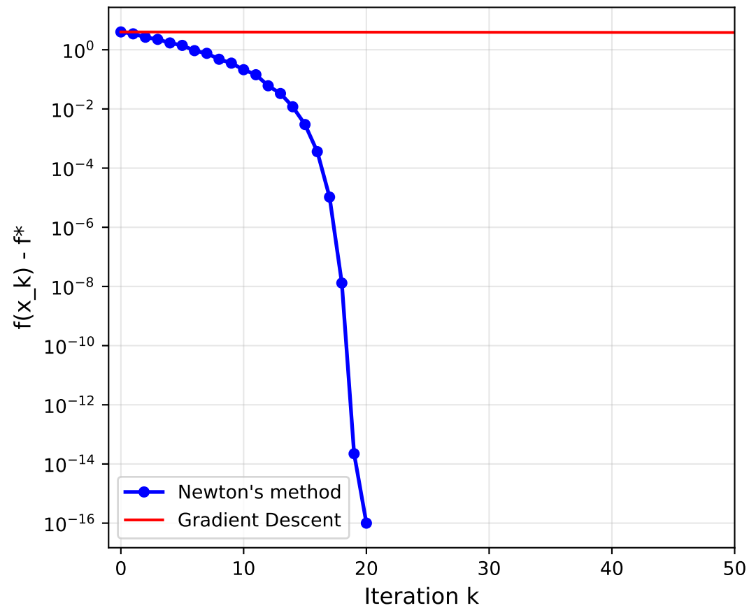
Newton's Method vs GD on Rosenbrock
