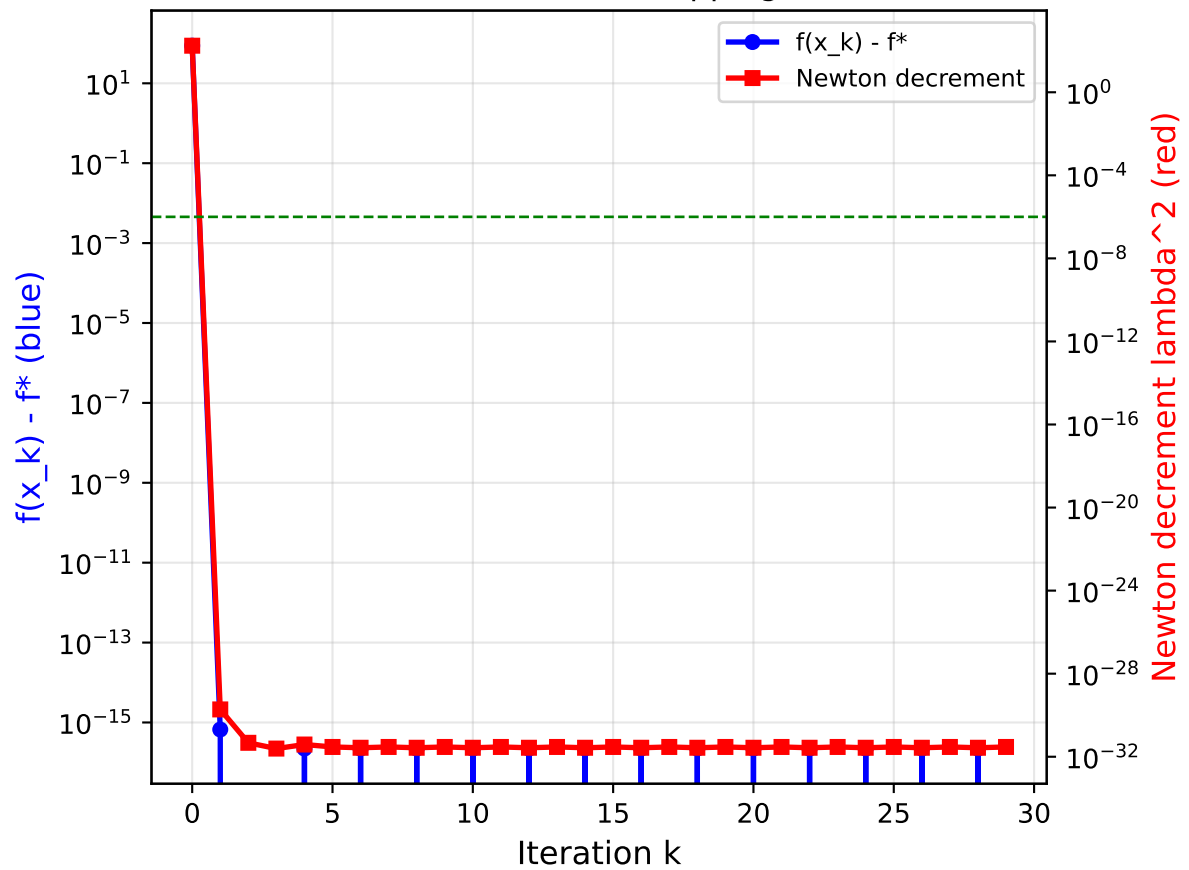
Newton Decrement as Stopping Criterion
