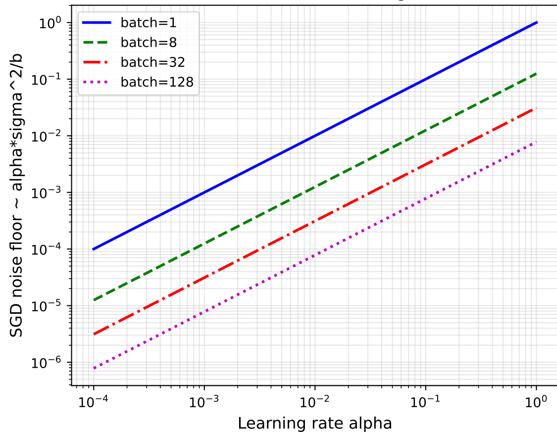
SGD Noise Floor vs Learning Rate
