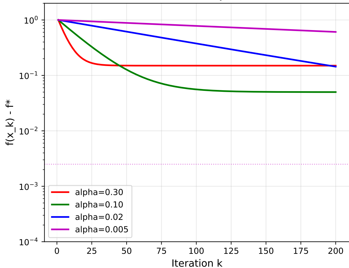
SGD: Deterministic Decay vs Noise Floor
