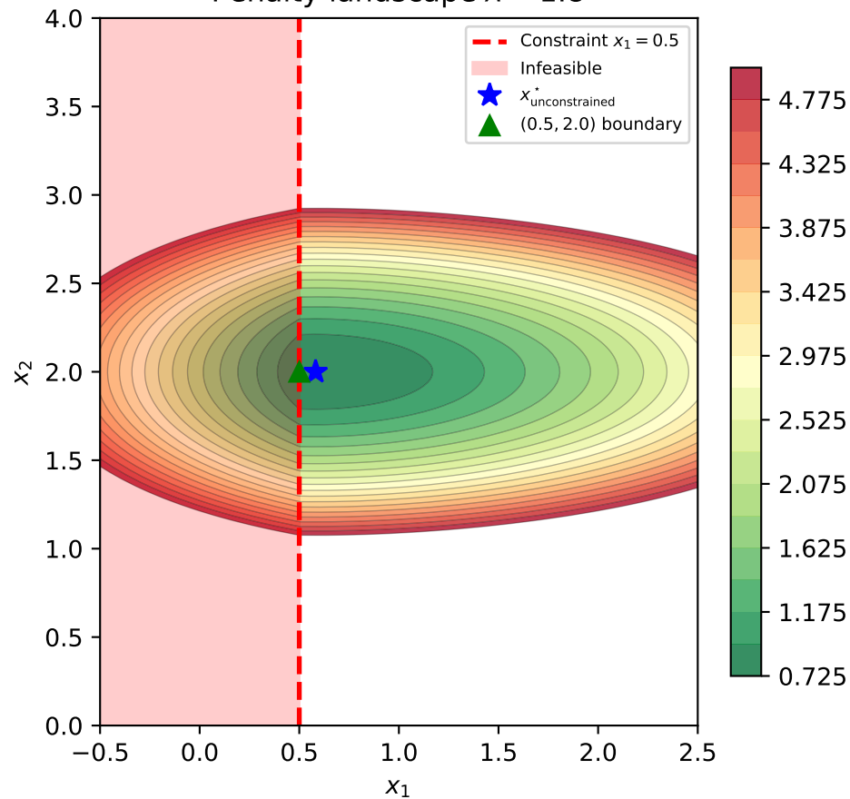
Penalty landscape \lambda = 1.8
