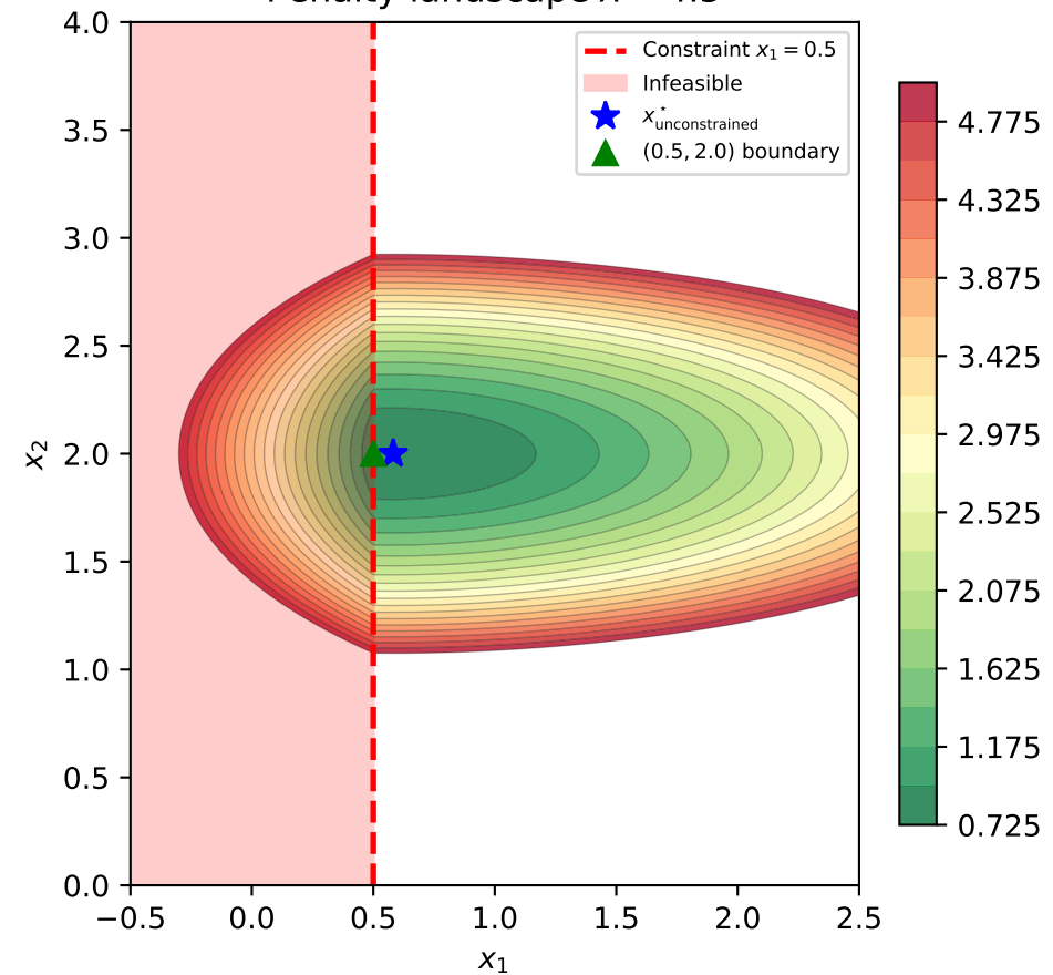
Penalty landscape \lambda = 4.5
