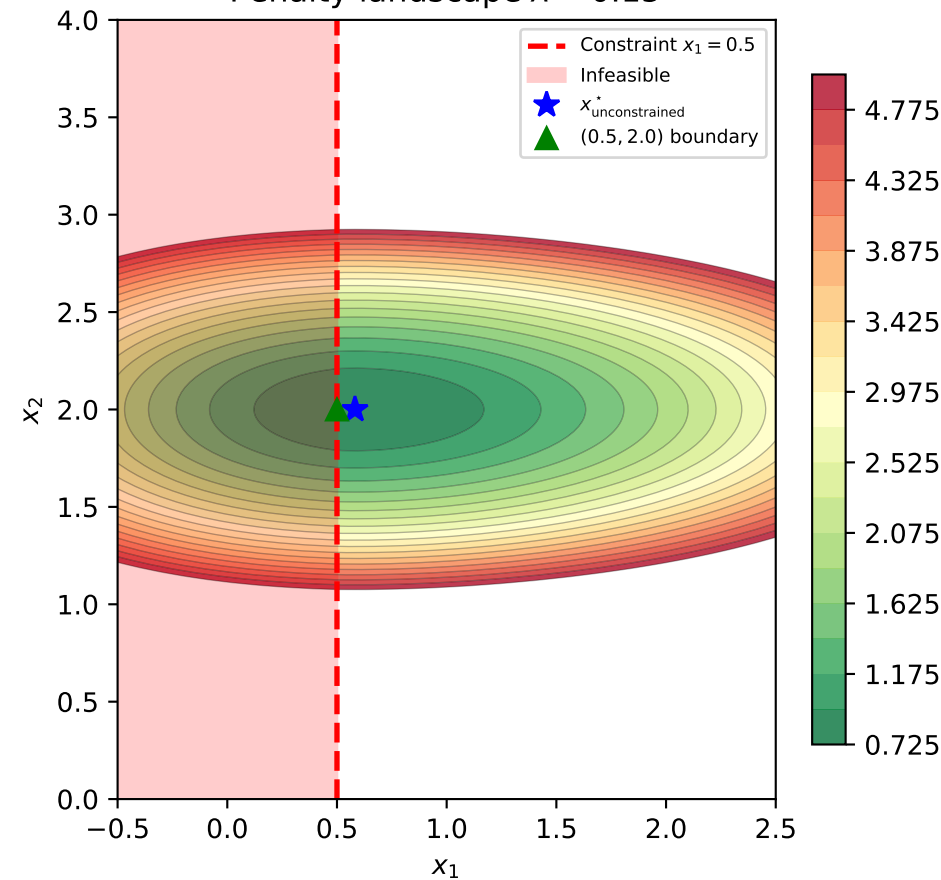
Penalty landscape \lambda = 0.15
