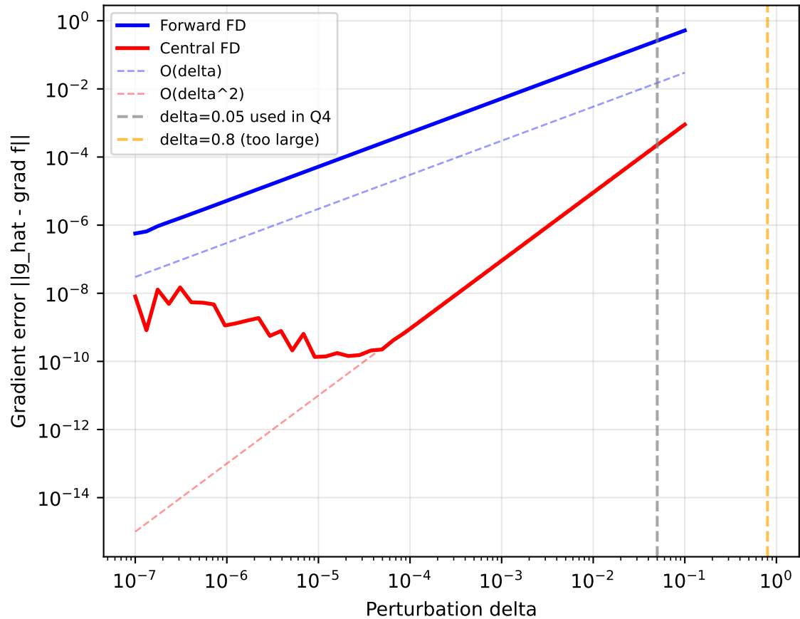
FD Gradient Error on Benchmark B
