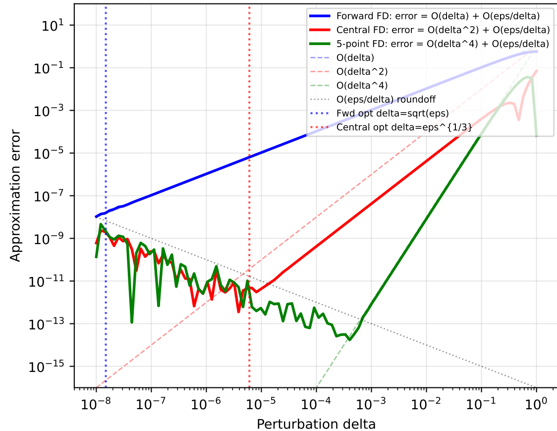
Finite Difference Error Analysis
