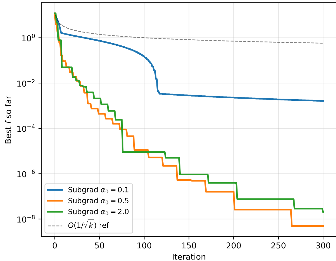
Subgradient: Effect of Step-Size Constant
