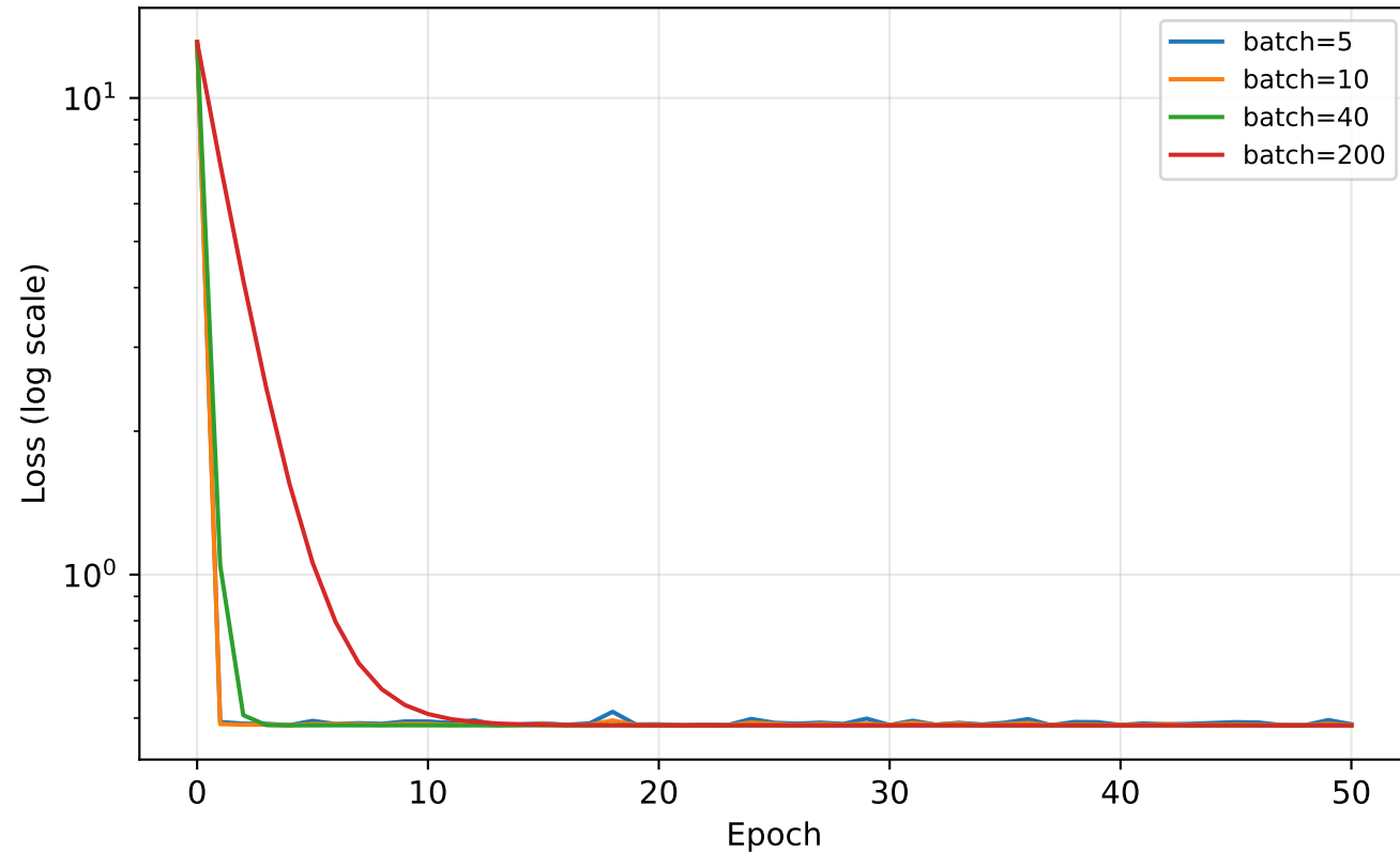
Mini-batch SGD: Learning rate \alpha = 0.06
