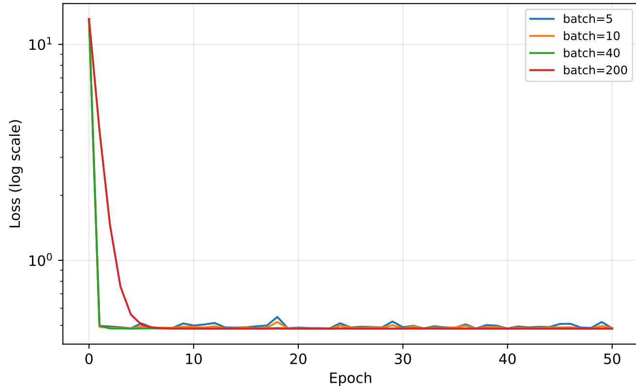
Mini-batch SGD: Learning rate \alpha = 0.12
