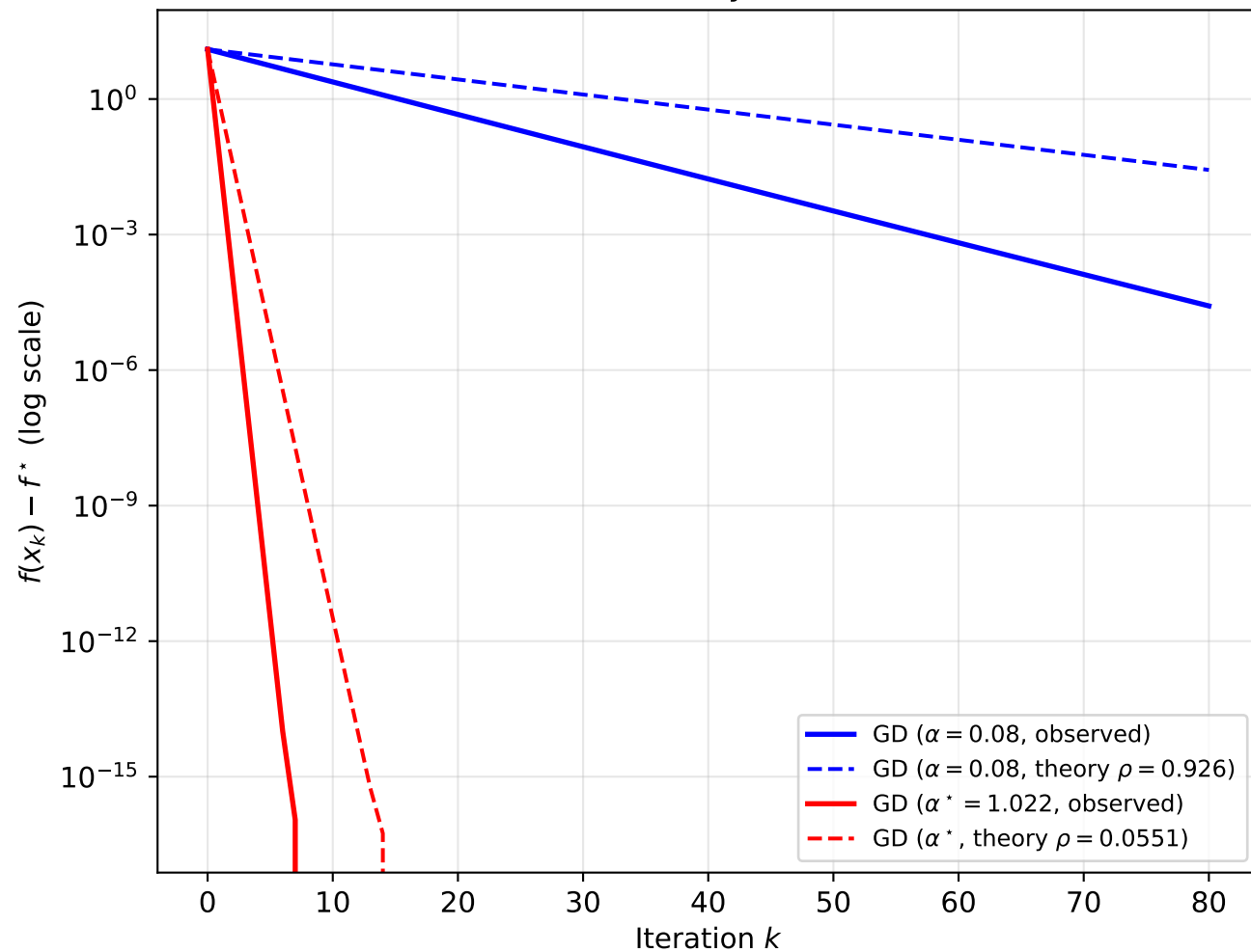
Benchmark A: Theory vs Practice (GD)
