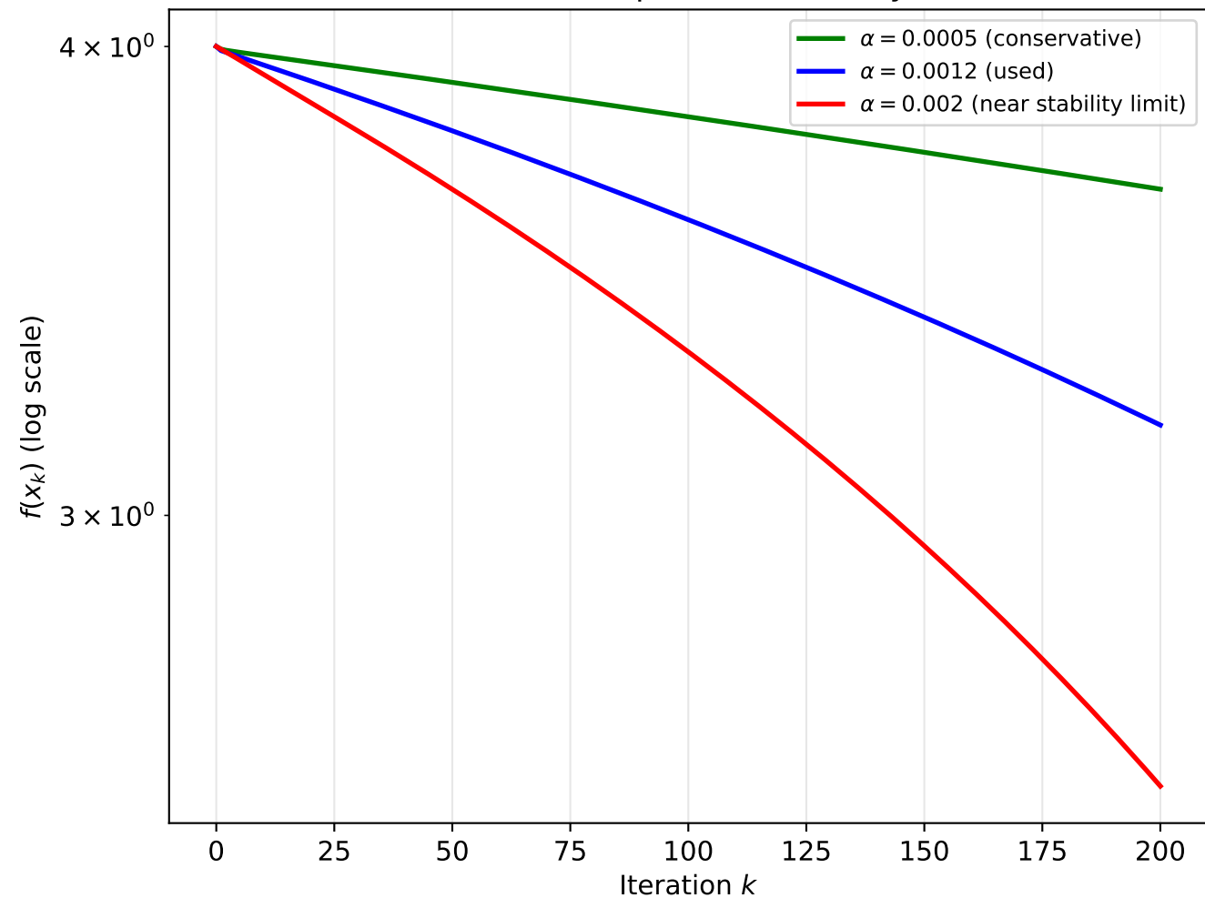
Benchmark C: GD Step Size Sensitivity (200 iters)
