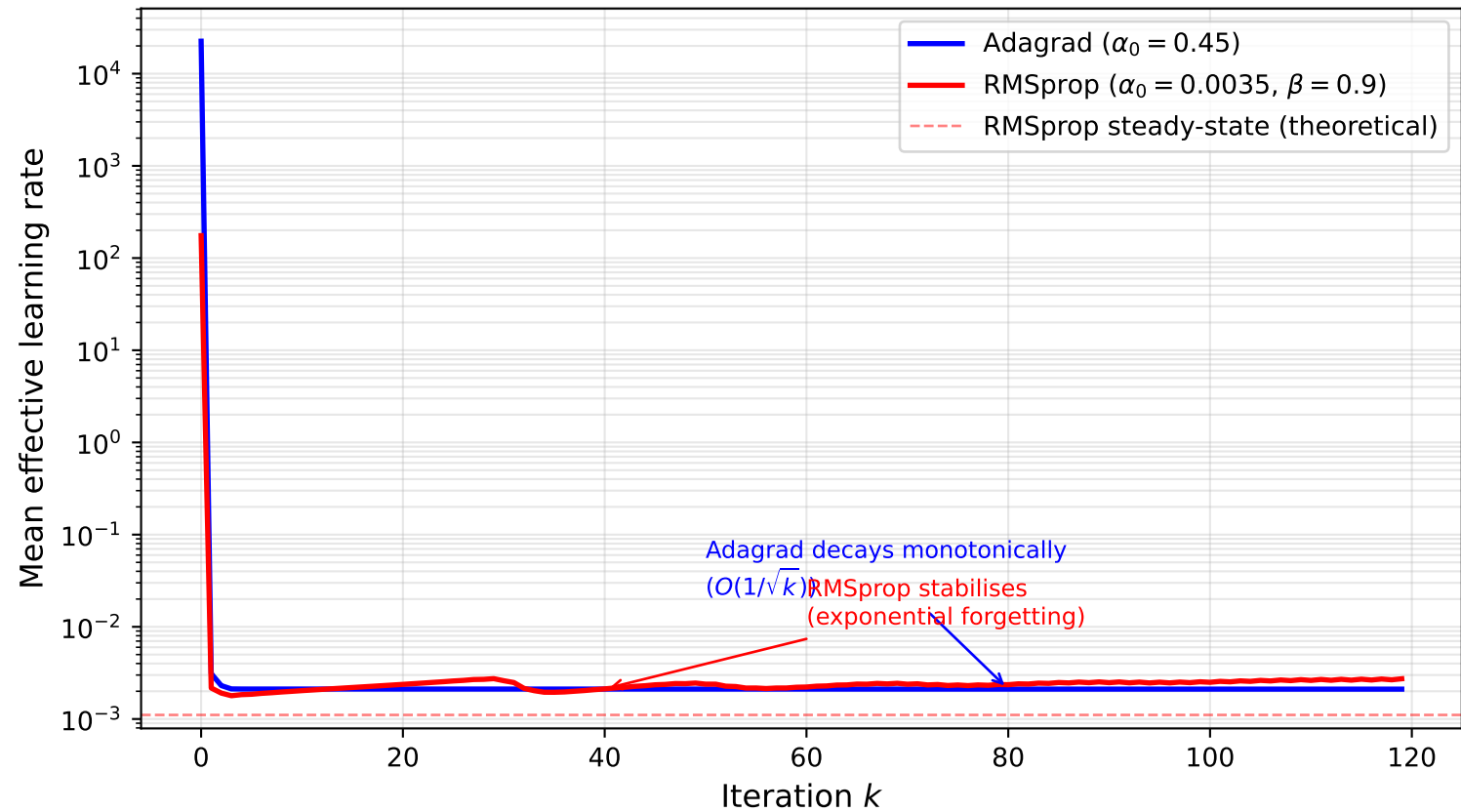
Adagrad vs. RMSprop: effective learning rate on Rosenbrock (Benchmark C)
