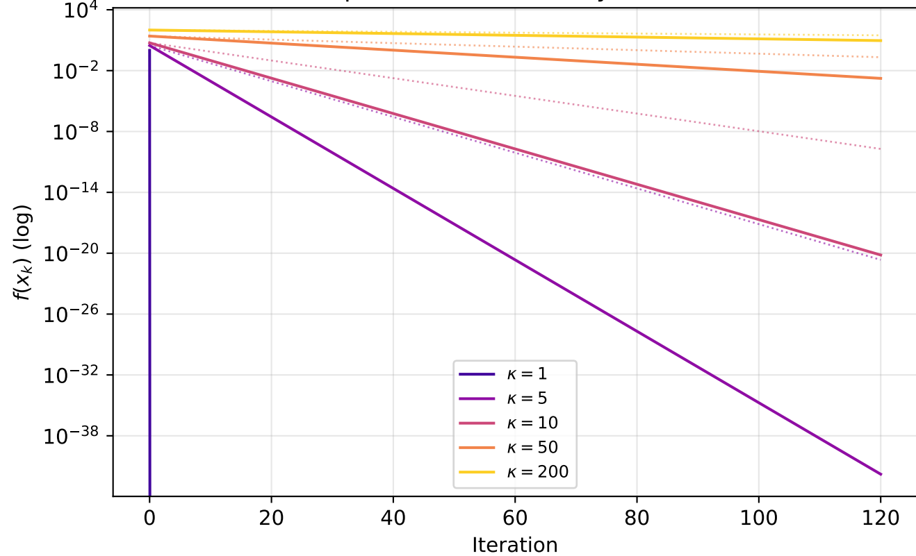
GD Convergence vs Condition Number \kappa (solid: empirical, dotted: theory (1 - 2/(\kappa + 1))^k )
