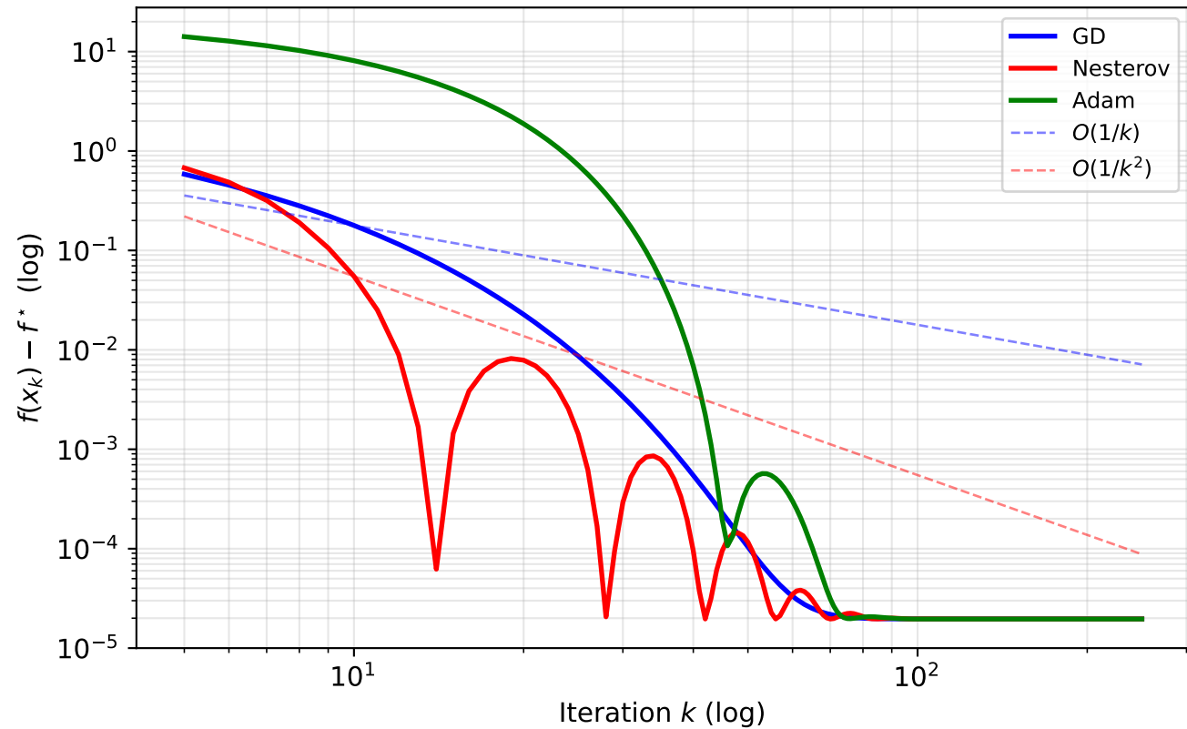
Convergence Rates on Benchmark B (log-log plot)
