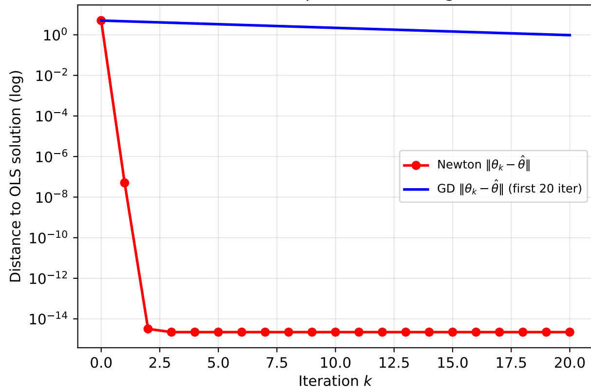
Q3: Newton's Method — Distance to OLS Solution Benchmark A: quadratic convergence
