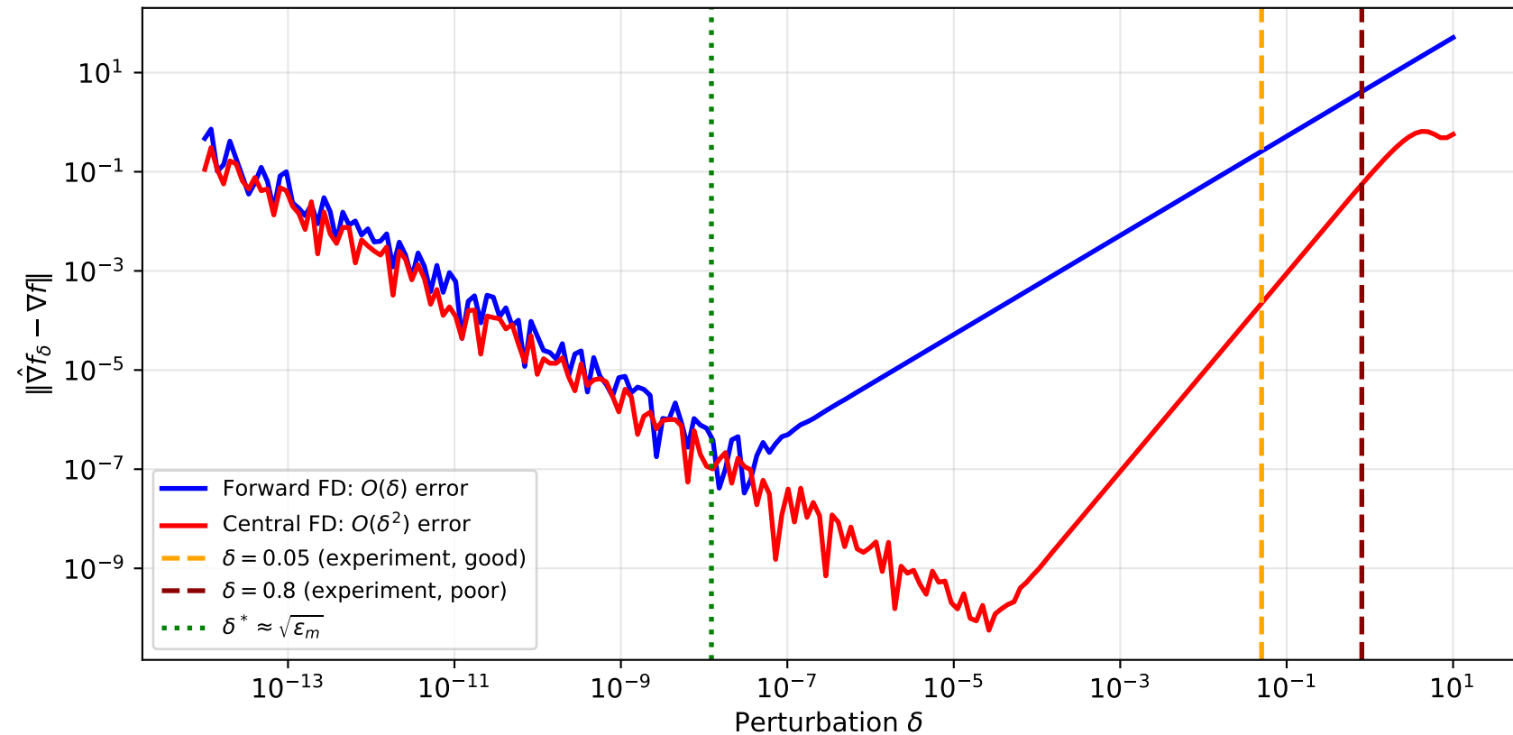
Q4: Forward vs Central FD Approximation Error Benchmark B evaluated at x_0 = (-1, 4)
