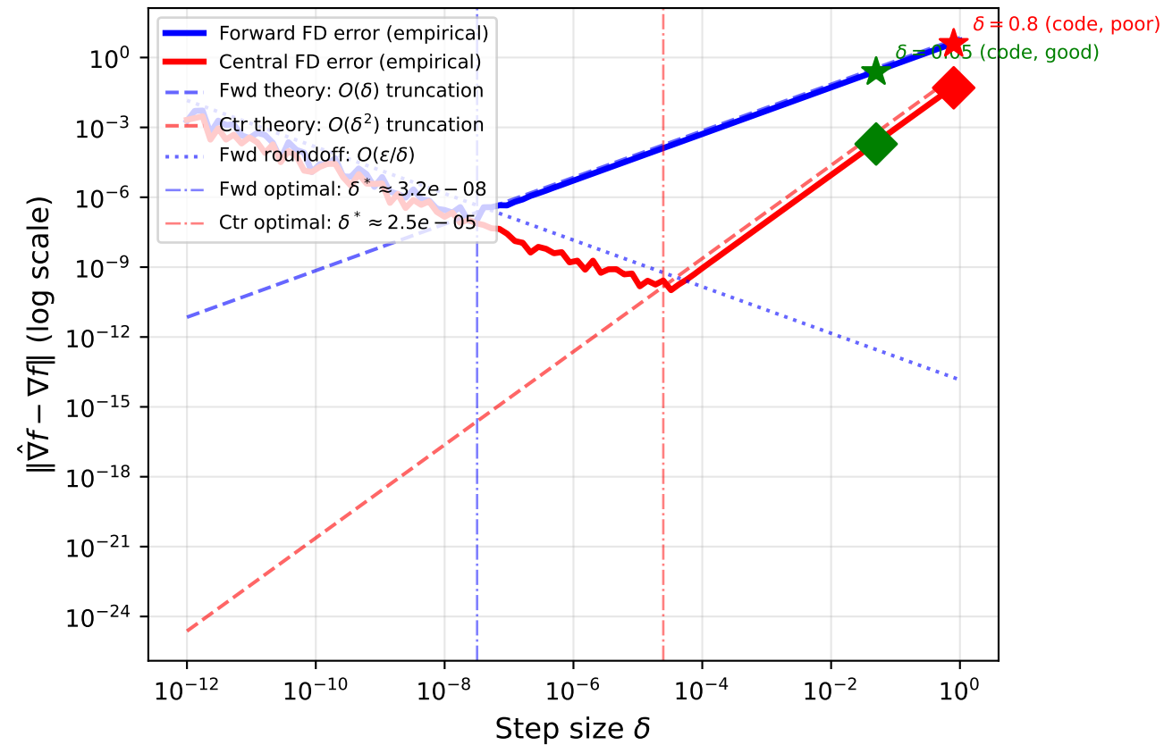
Finite Difference Error vs Step Size \delta (Benchmark B at x_0 = (-1, 4) )
