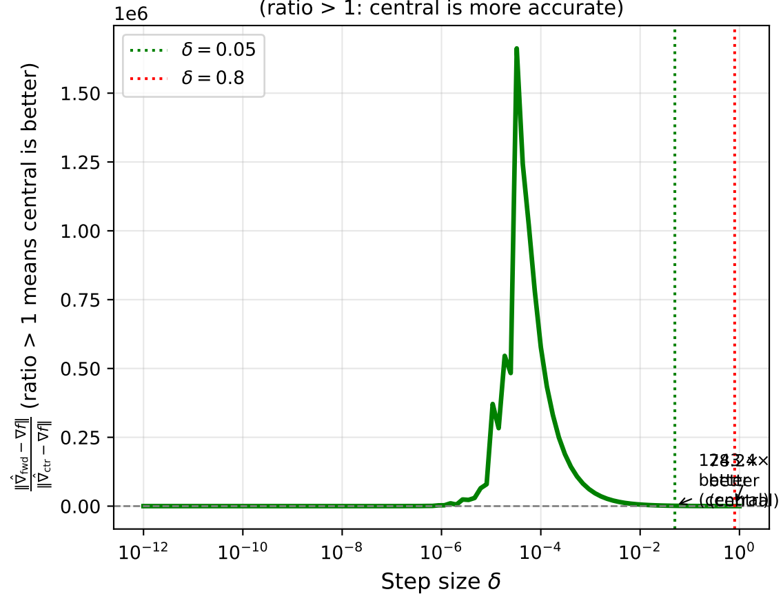
Central vs Forward FD Accuracy Ratio (ratio > 1: central is more accurate)
