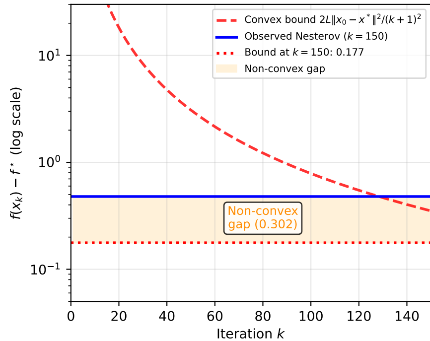
Non-convex deviation: Rosenbrock
