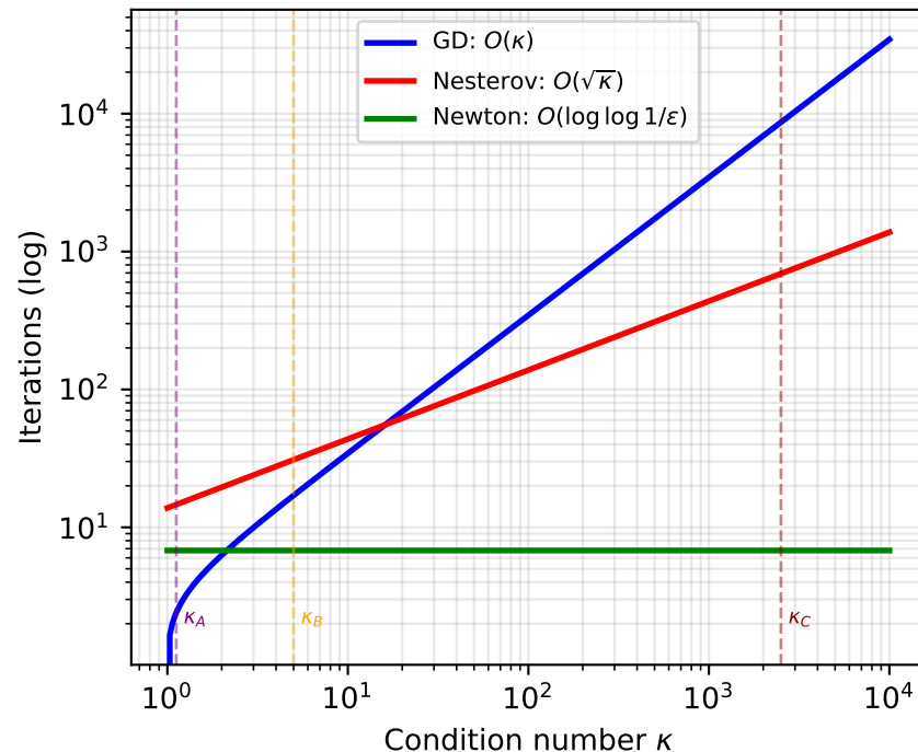
Iterations to \varepsilon = 10^{-6} accuracy
