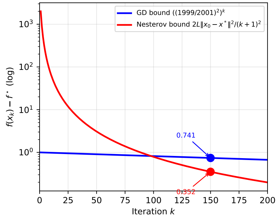
Theoretical bounds ( \kappa = 2000 , convex)
