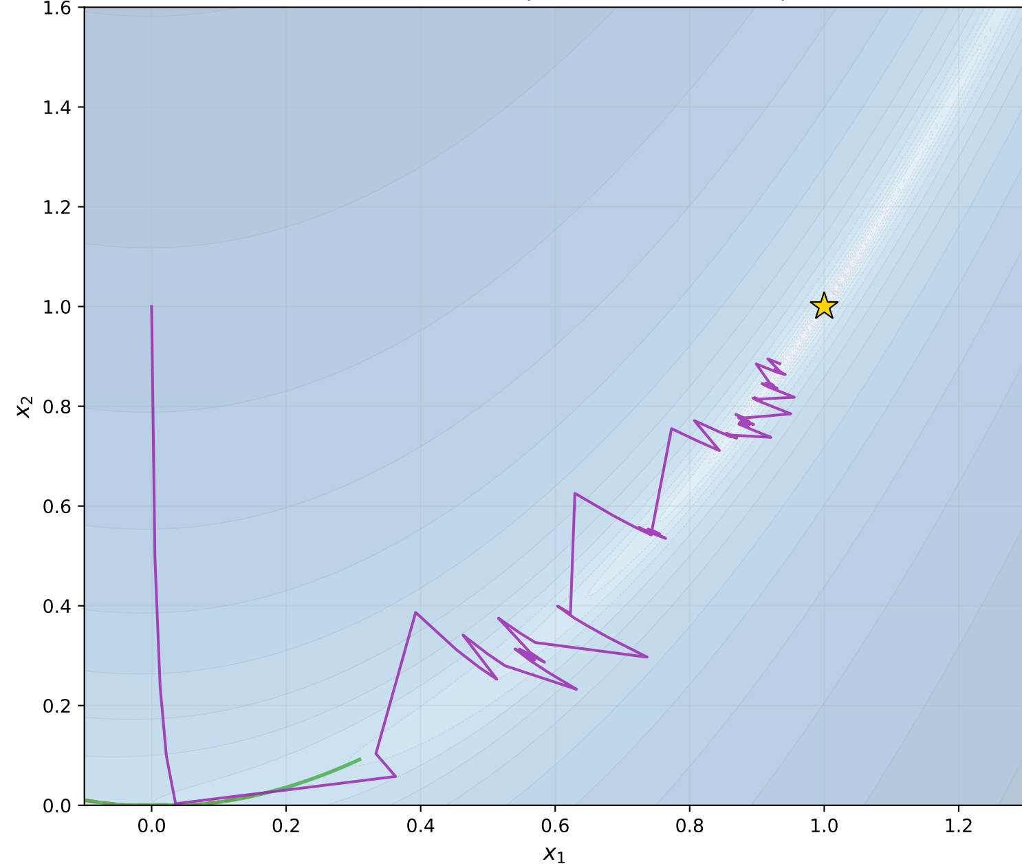
All Methods: Rosenbrock Trajectories (zoomed near optimum)
