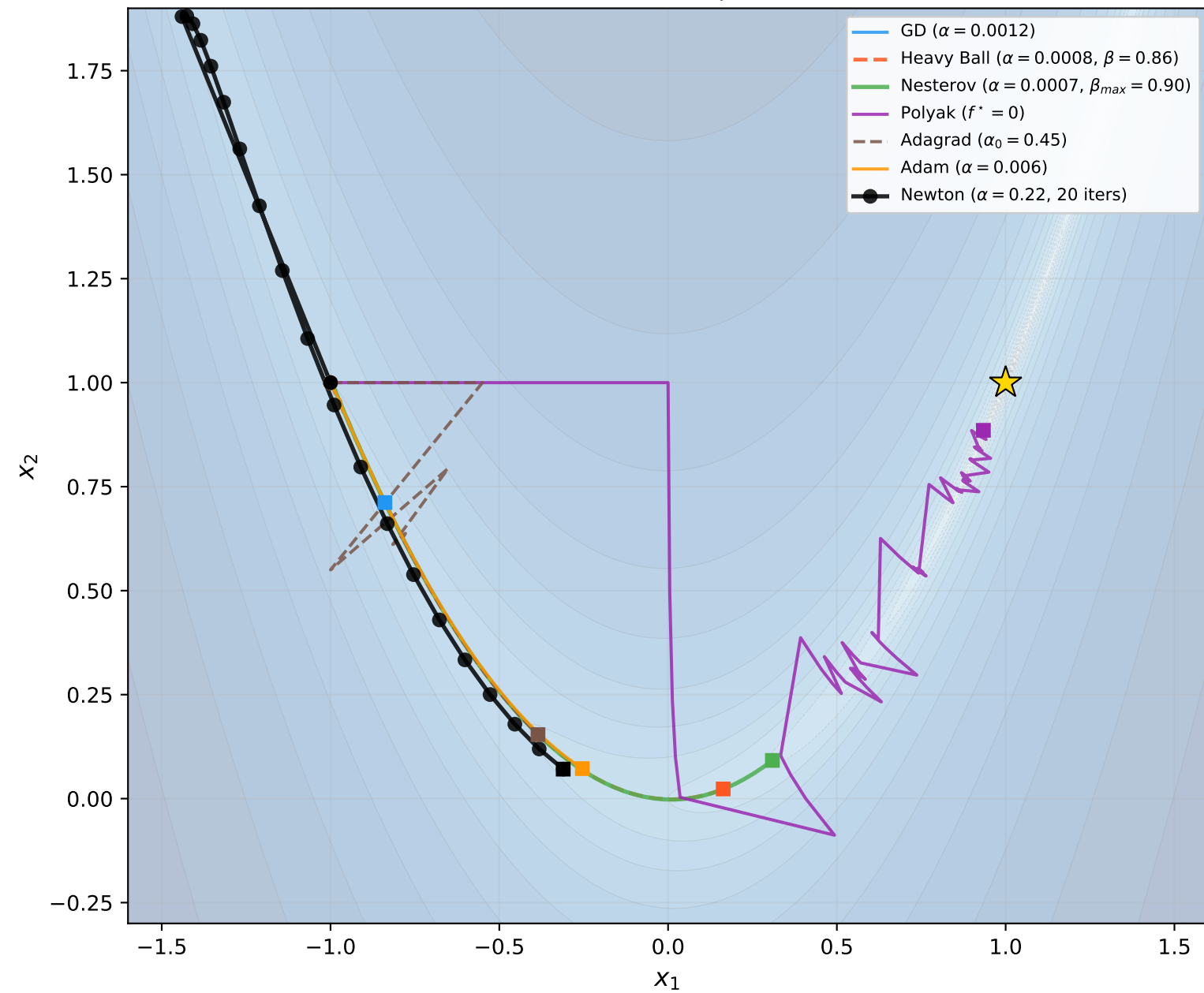
All Methods: Rosenbrock Trajectories (full view)
