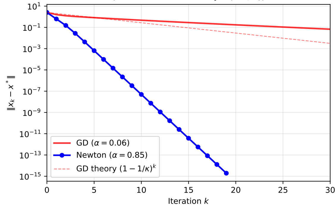
Convergence: Newton vs GD (Benchmark B from x_0 = (-1, 4) )
