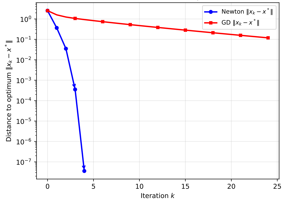
Newton vs GD: Distance to Optimum
