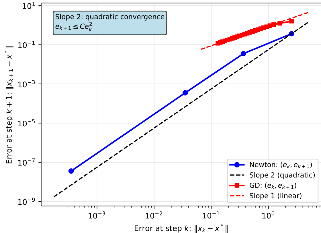
Quadratic Convergence: e_{k+1} vs e_k (log-log)
